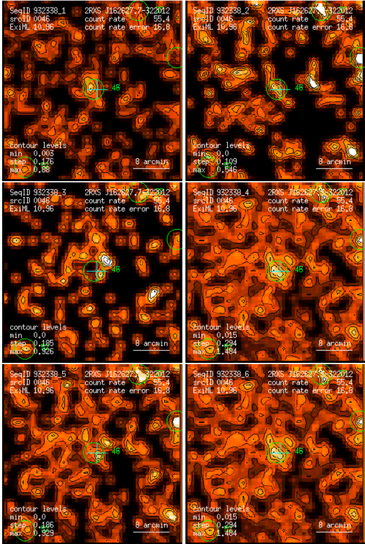
Figure 46: RASS 932338: detection 0046: band rate images, Gaussian filter: (1) PSPC channels 11 – 41, (2) 52 – 90, (3) 91 – 201, (4) 11 – 235, (5) 52 – 201, (6) 11 – 201. Broad band rates in counts/ks. Band rate contour levels in counts/ks/arcmin 2 .
