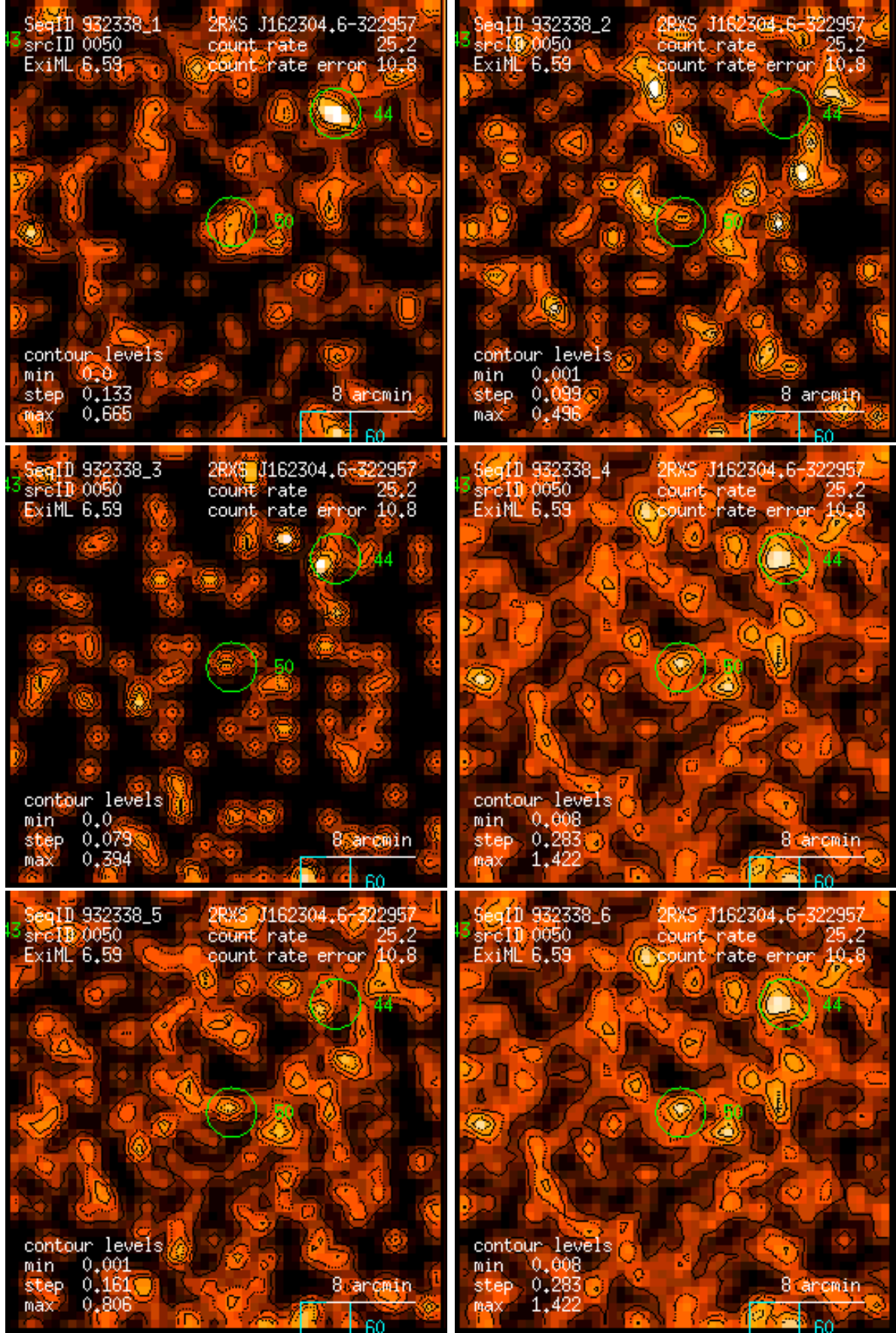
Figure 50: RASS 932338: detection 0050: band rate images, Gaussian filter: (1) PSPC channels 11 – 41, (2) 52 – 90, (3) 91 – 201, (4) 11 – 235, (5) 52 – 201, (6) 11 – 201. Broad band rates in counts/ks. Band rate contour levels in counts/ks/arcmin 2 .
