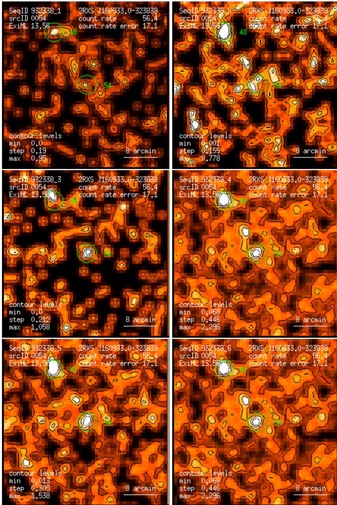
Figure 54: RASS 932338: detection 0054: band rate images, Gaussian filter: (1) PSPC channels 11 – 41, (2) 52 – 90, (3) 91 – 201, (4) 11 – 235, (5) 52 – 201, (6) 11 – 201. Broad band rates in counts/ks. Band rate contour levels in counts/ks/arcmin 2 .
