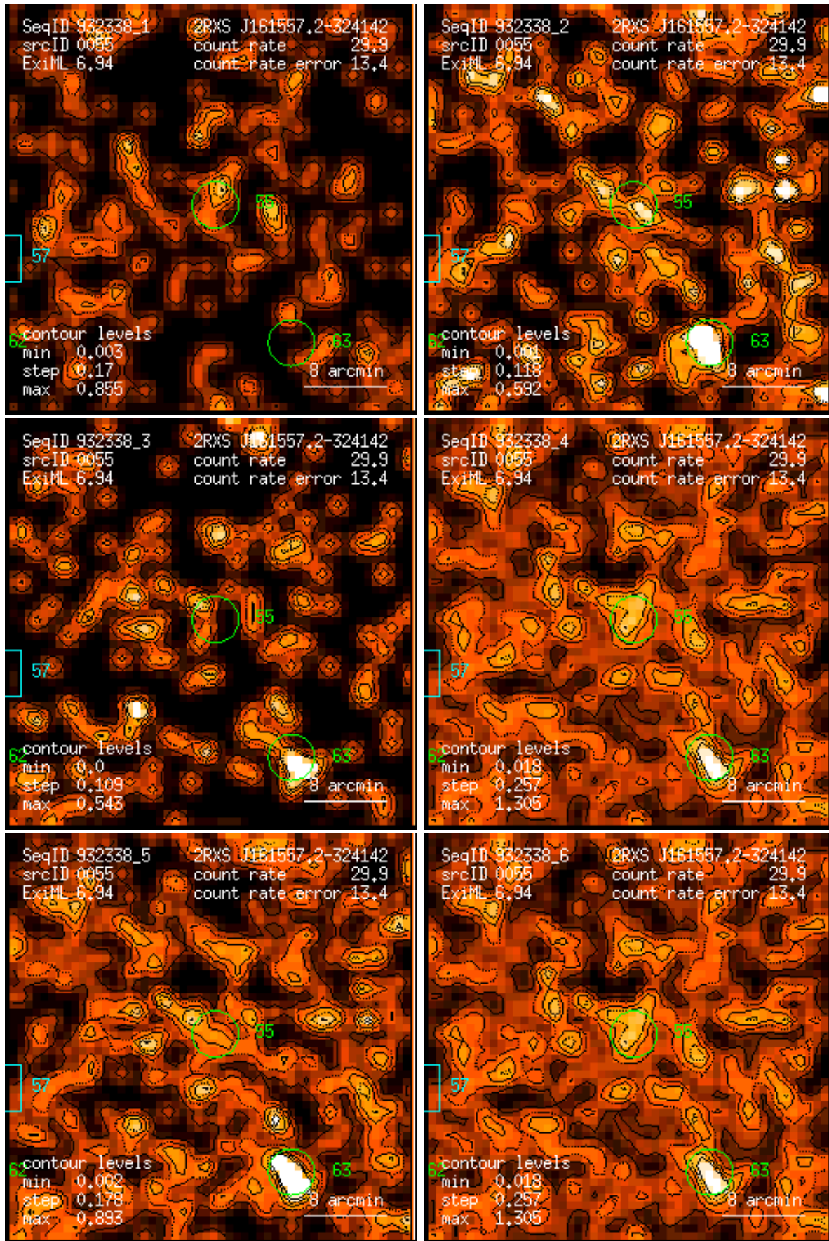
Figure 55: RASS 932338: detection 0055: band rate images, Gaussian filter: (1) PSPC channels 11 – 41, (2) 52 – 90, (3) 91 – 201, (4) 11 – 235, (5) 52 – 201, (6) 11 – 201. Broad band rates in counts/ks. Band rate contour levels in counts/ks/arcmin 2 .
