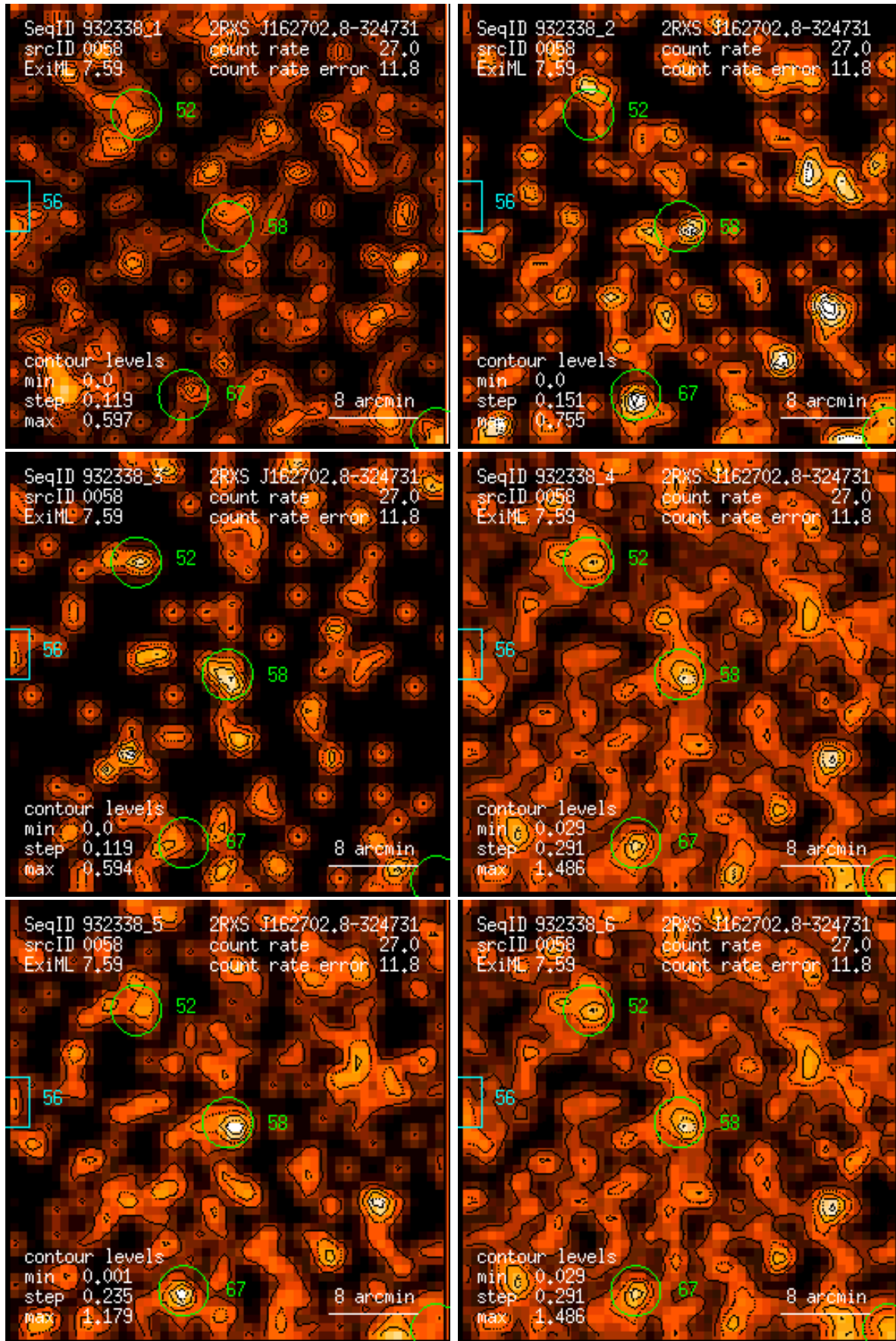
Figure 58: RASS 932338: detection 0058: band rate images, Gaussian filter: (1) PSPC channels 11 – 41, (2) 52 – 90, (3) 91 – 201, (4) 11 – 235, (5) 52 – 201, (6) 11 – 201. Broad band rates in counts/ks. Band rate contour levels in counts/ks/arcmin 2 .
