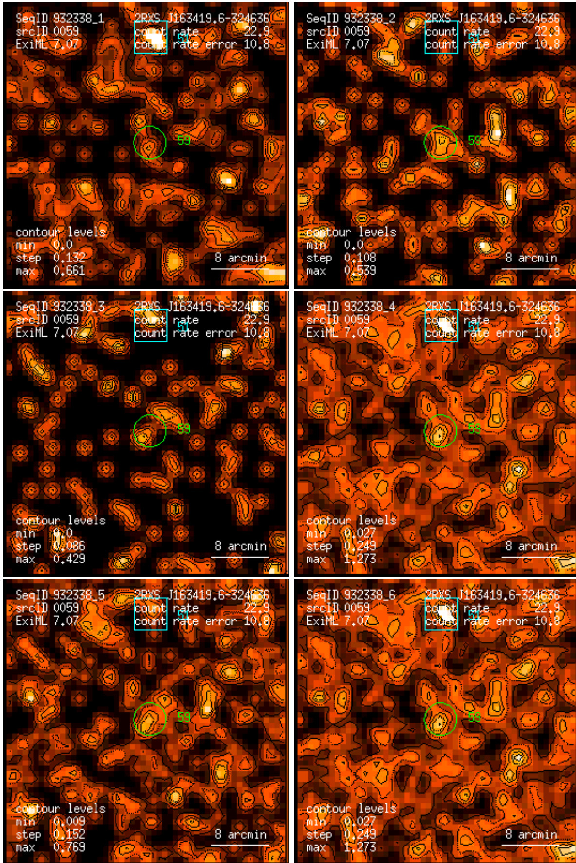
Figure 59: RASS 932338: detection 0059: band rate images, Gaussian filter: (1) PSPC channels 11 – 41, (2) 52 – 90, (3) 91 – 201, (4) 11 – 235, (5) 52 – 201, (6) 11 – 201. Broad band rates in counts/ks. Band rate contour levels in counts/ks/arcmin 2 .
