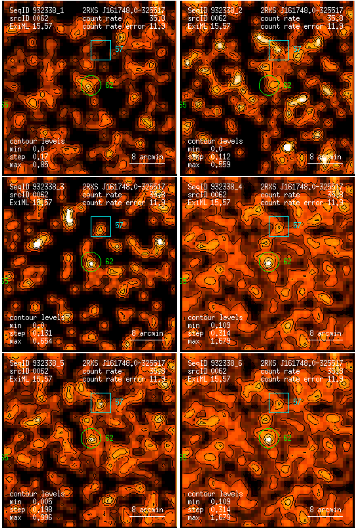
Figure 62: RASS 932338: detection 0062: band rate images, Gaussian filter: (1) PSPC channels 11 – 41, (2) 52 – 90, (3) 91 – 201, (4) 11 – 235, (5) 52 – 201, (6) 11 – 201. Broad band rates in counts/ks. Band rate contour levels in counts/ks/arcmin 2 .
