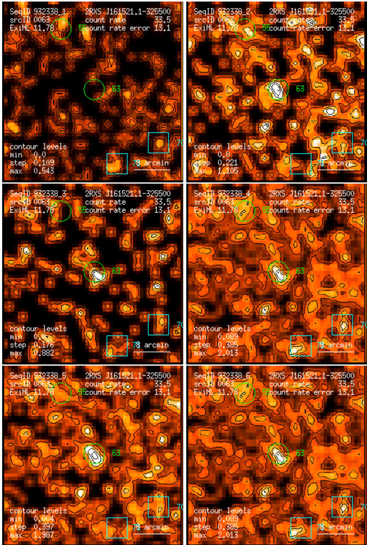
Figure 63: RASS 932338: detection 0063: band rate images, Gaussian filter: (1) PSPC channels 11 – 41, (2) 52 – 90, (3) 91 – 201, (4) 11 – 235, (5) 52 – 201, (6) 11 – 201. Broad band rates in counts/ks. Band rate contour levels in counts/ks/arcmin 2 .
