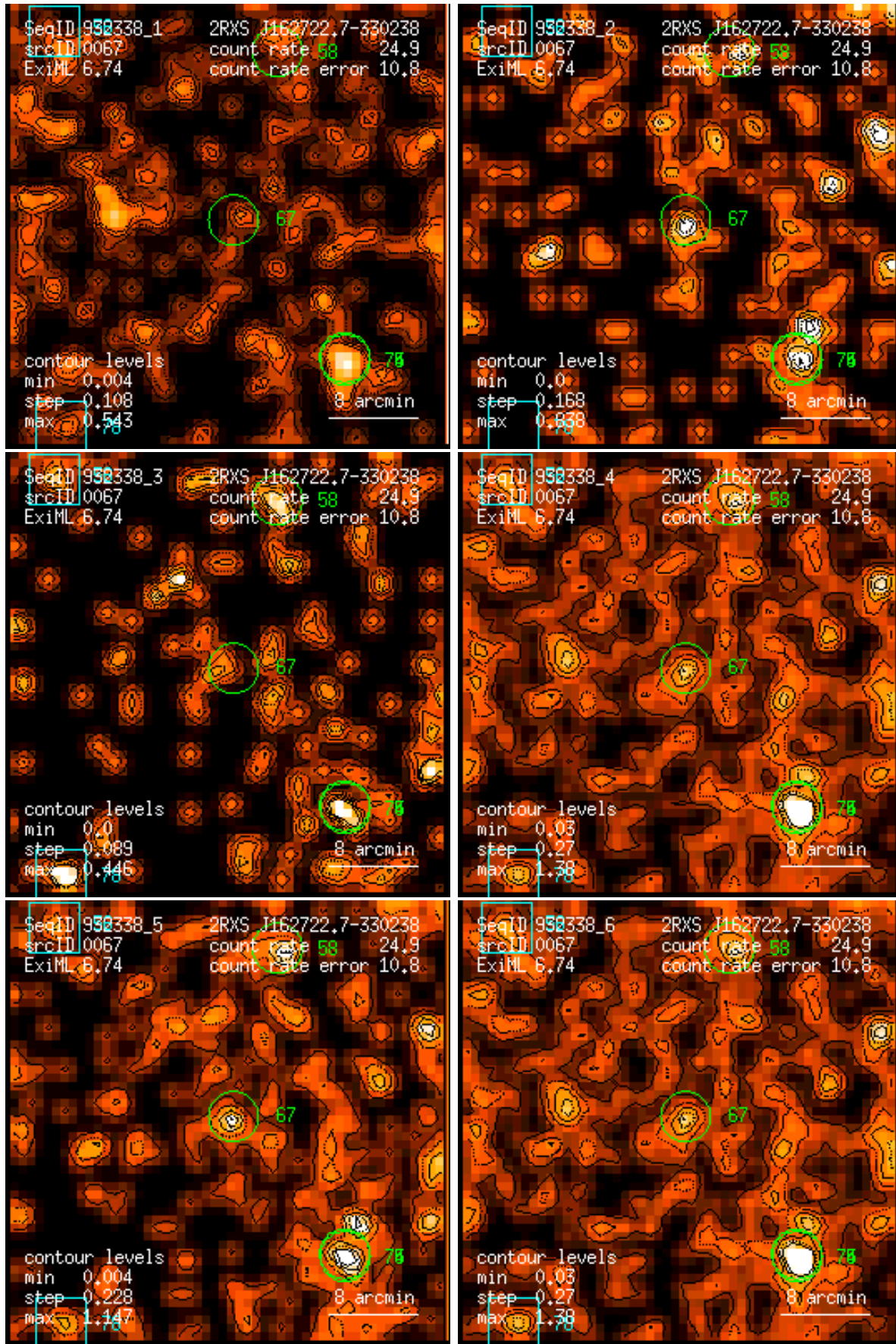
Figure 67: RASS 932338: detection 0067: band rate images, Gaussian filter: (1) PSPC channels 11 – 41, (2) 52 – 90, (3) 91 – 201, (4) 11 – 235, (5) 52 – 201, (6) 11 – 201. Broad band rates in counts/ks. Band rate contour levels in counts/ks/arcmin 2 .
