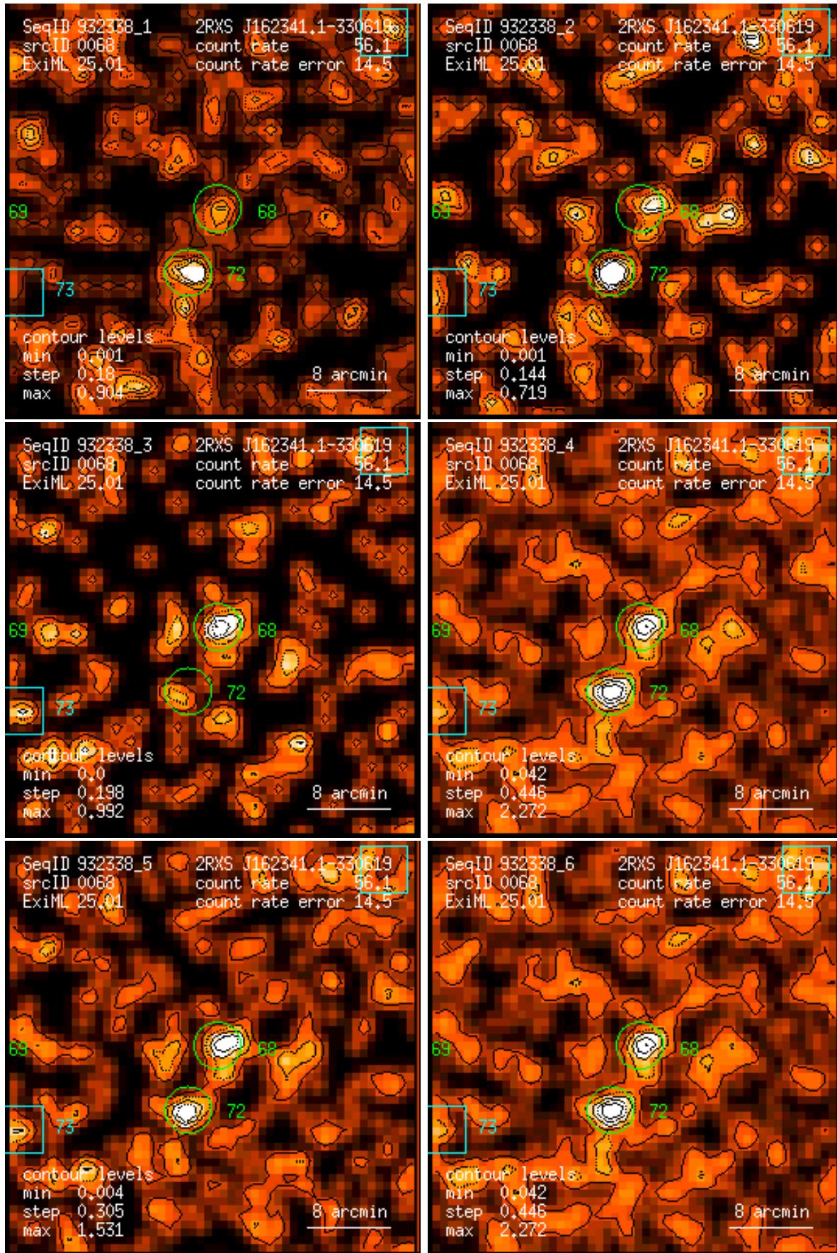
Figure 68: RASS 932338: detection 0068: band rate images, Gaussian filter: (1) PSPC channels 11 – 41, (2) 52 – 90, (3) 91 – 201, (4) 11 – 235, (5) 52 – 201, (6) 11 – 201. Broad band rates in counts/ks. Band rate contour levels in counts/ks/arcmin 2 .
