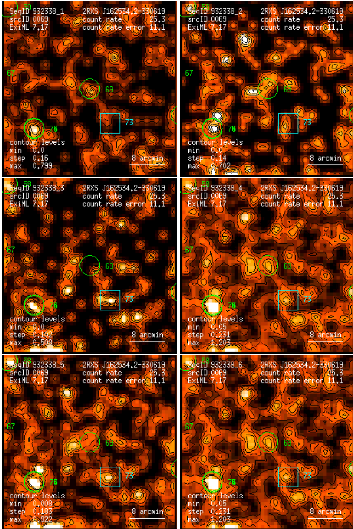
Figure 69: RASS 932338: detection 0069: band rate images, Gaussian filter: (1) PSPC channels 11 – 41, (2) 52 – 90, (3) 91 – 201, (4) 11 – 235, (5) 52 – 201, (6) 11 – 201. Broad band rates in counts/ks. Band rate contour levels in counts/ks/arcmin 2 .
