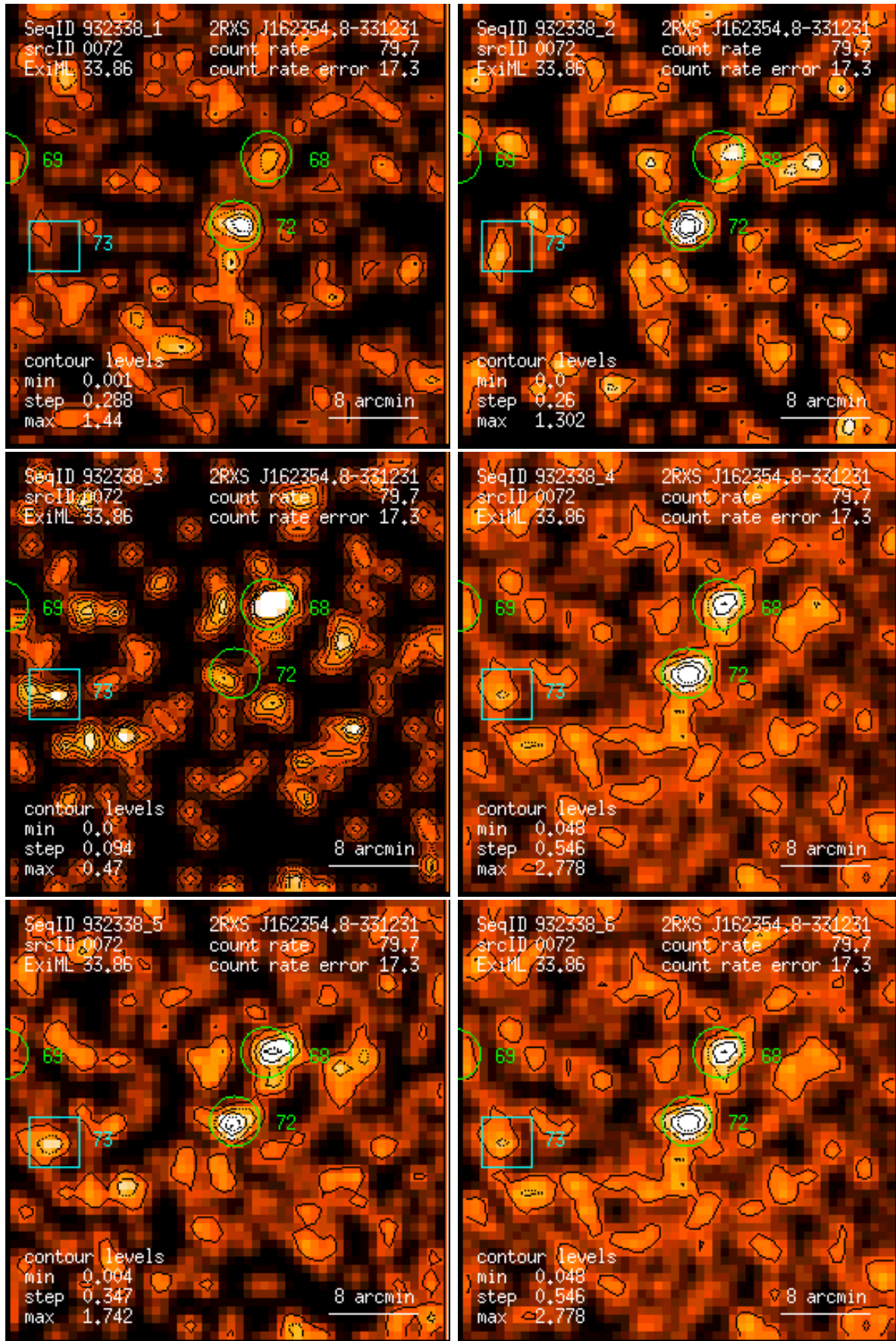
Figure 72: RASS 932338: detection 0072: band rate images, Gaussian filter: (1) PSPC channels 11 – 41, (2) 52 – 90, (3) 91 – 201, (4) 11 – 235, (5) 52 – 201, (6) 11 – 201. Broad band rates in counts/ks. Band rate contour levels in counts/ks/arcmin 2 .
