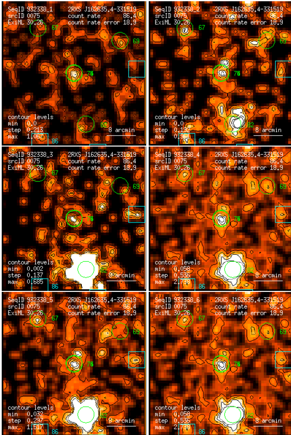
Figure 75: RASS 932338: detection 0075: band rate images, Gaussian filter: (1) PSPC channels 11 – 41, (2) 52 – 90, (3) 91 – 201, (4) 11 – 235, (5) 52 – 201, (6) 11 – 201. Broad band rates in counts/ks. Band rate contour levels in counts/ks/arcmin 2 .
