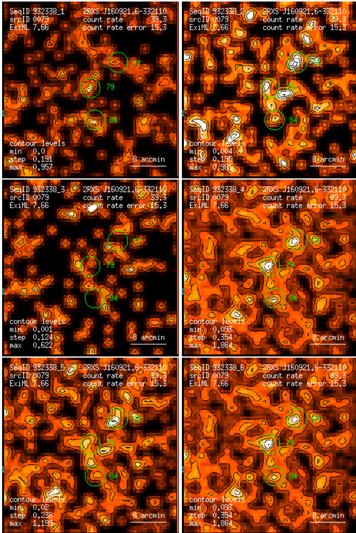
Figure 79: RASS 932338: detection 0079: band rate images, Gaussian filter: (1) PSPC channels 11 – 41, (2) 52 – 90, (3) 91 – 201, (4) 11 – 235, (5) 52 – 201, (6) 11 – 201. Broad band rates in counts/ks. Band rate contour levels in counts/ks/arcmin 2 .
