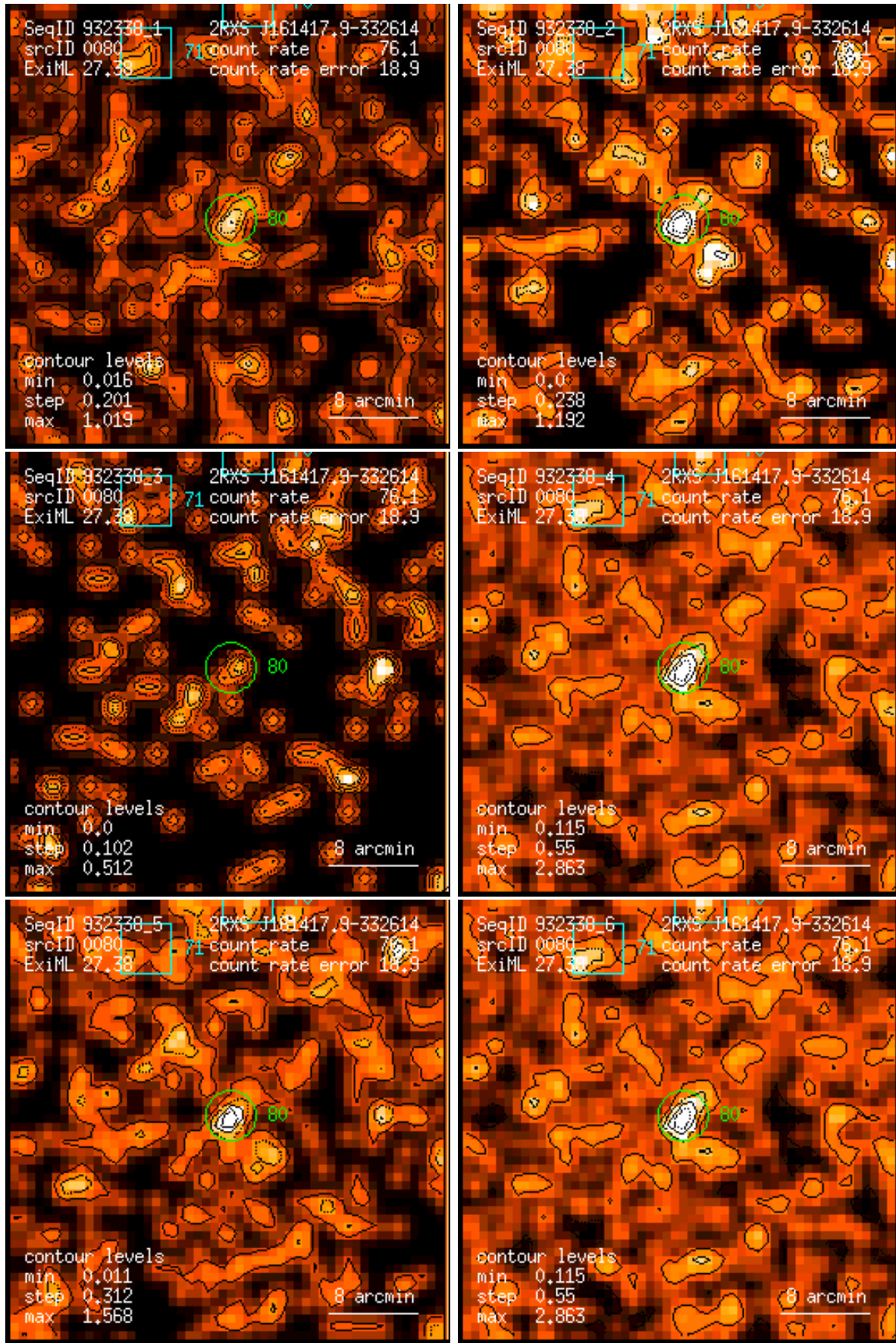
Figure 80: RASS 932338: detection 0080: band rate images, Gaussian filter: (1) PSPC channels 11 – 41, (2) 52 – 90, (3) 91 – 201, (4) 11 – 235, (5) 52 – 201, (6) 11 – 201. Broad band rates in counts/ks. Band rate contour levels in counts/ks/arcmin 2 .
