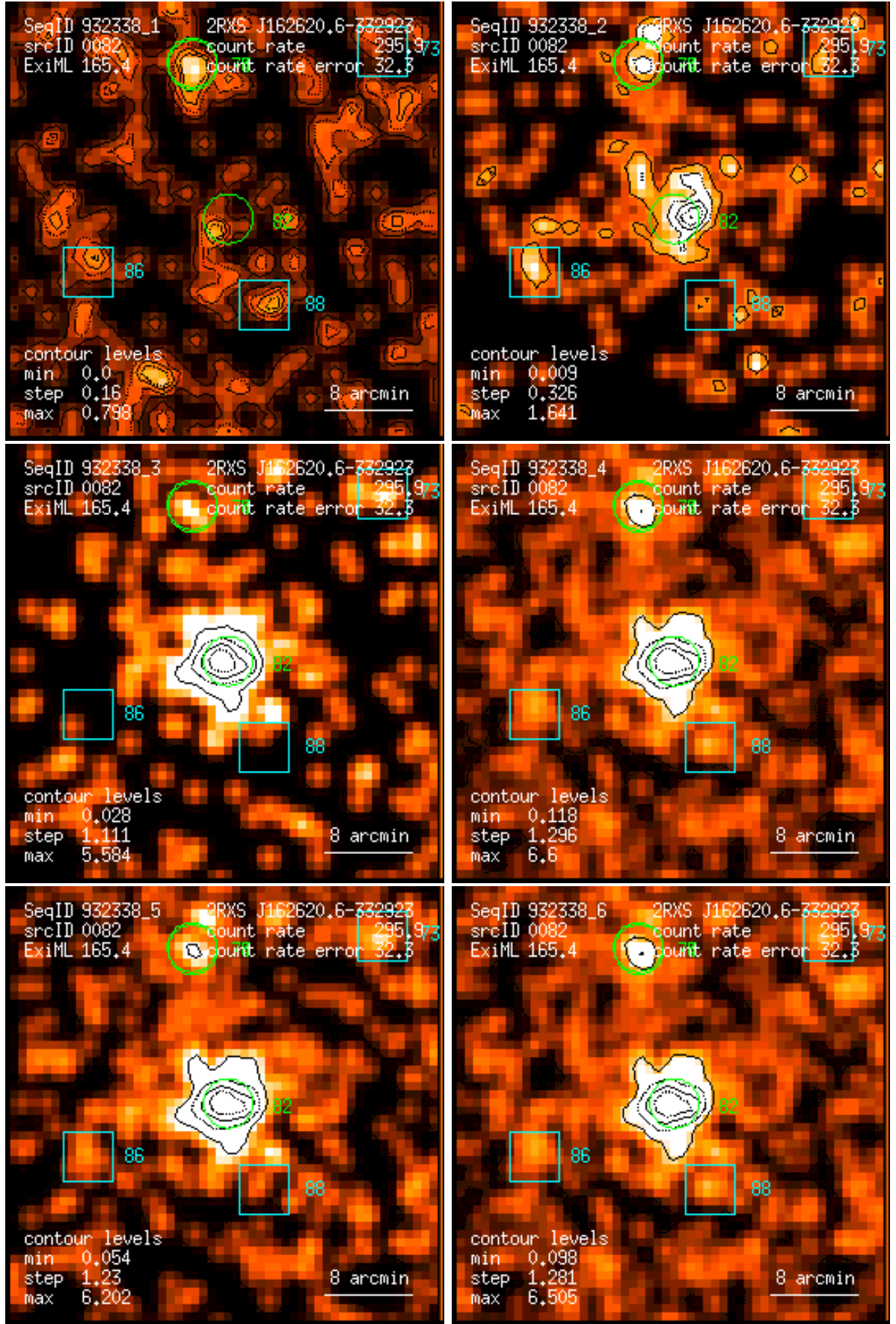
Figure 82: RASS 932338: detection 0082: band rate images, Gaussian filter: (1) PSPC channels 11 – 41, (2) 52 – 90, (3) 91 – 201, (4) 11 – 235, (5) 52 – 201, (6) 11 – 201. Broad band rates in counts/ks. Band rate contour levels in counts/ks/arcmin 2 .
