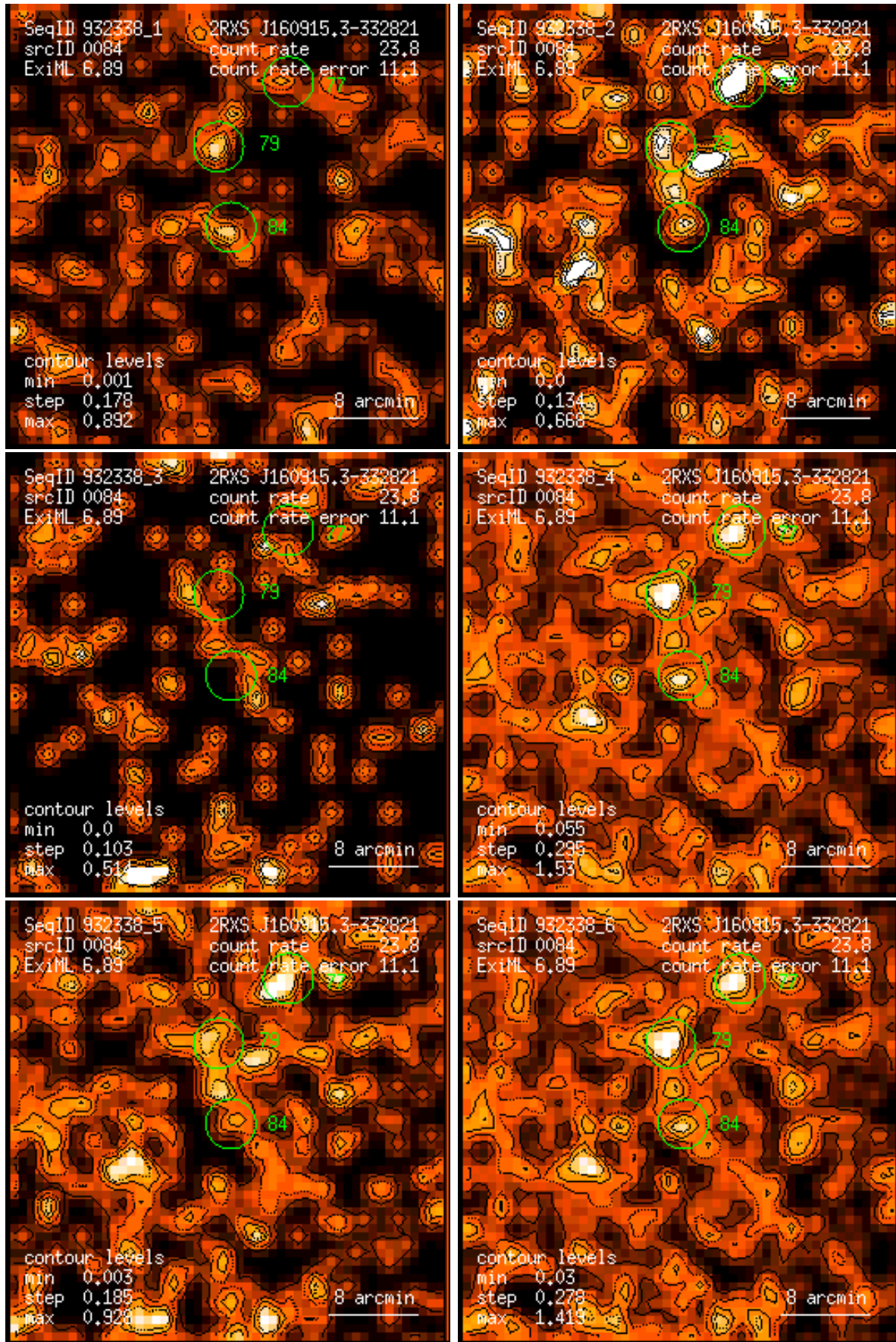
Figure 84: RASS 932338: detection 0084: band rate images, Gaussian filter: (1) PSPC channels 11 – 41, (2) 52 – 90, (3) 91 – 201, (4) 11 – 235, (5) 52 – 201, (6) 11 – 201. Broad band rates in counts/ks. Band rate contour levels in counts/ks/arcmin 2 .
