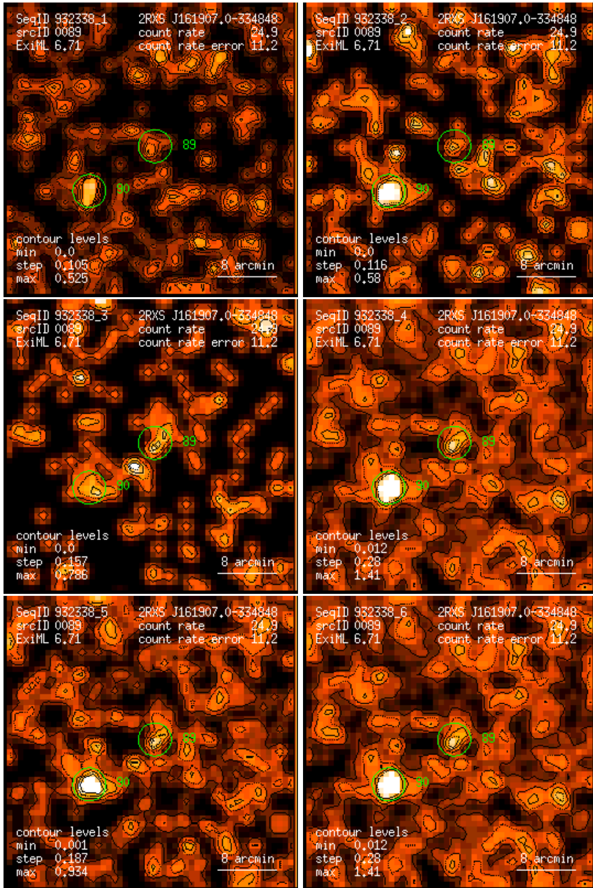
Figure 89: RASS 932338: detection 0089: band rate images, Gaussian filter: (1) PSPC channels 11 – 41, (2) 52 – 90, (3) 91 – 201, (4) 11 – 235, (5) 52 – 201, (6) 11 – 201. Broad band rates in counts/ks. Band rate contour levels in counts/ks/arcmin 2 .
