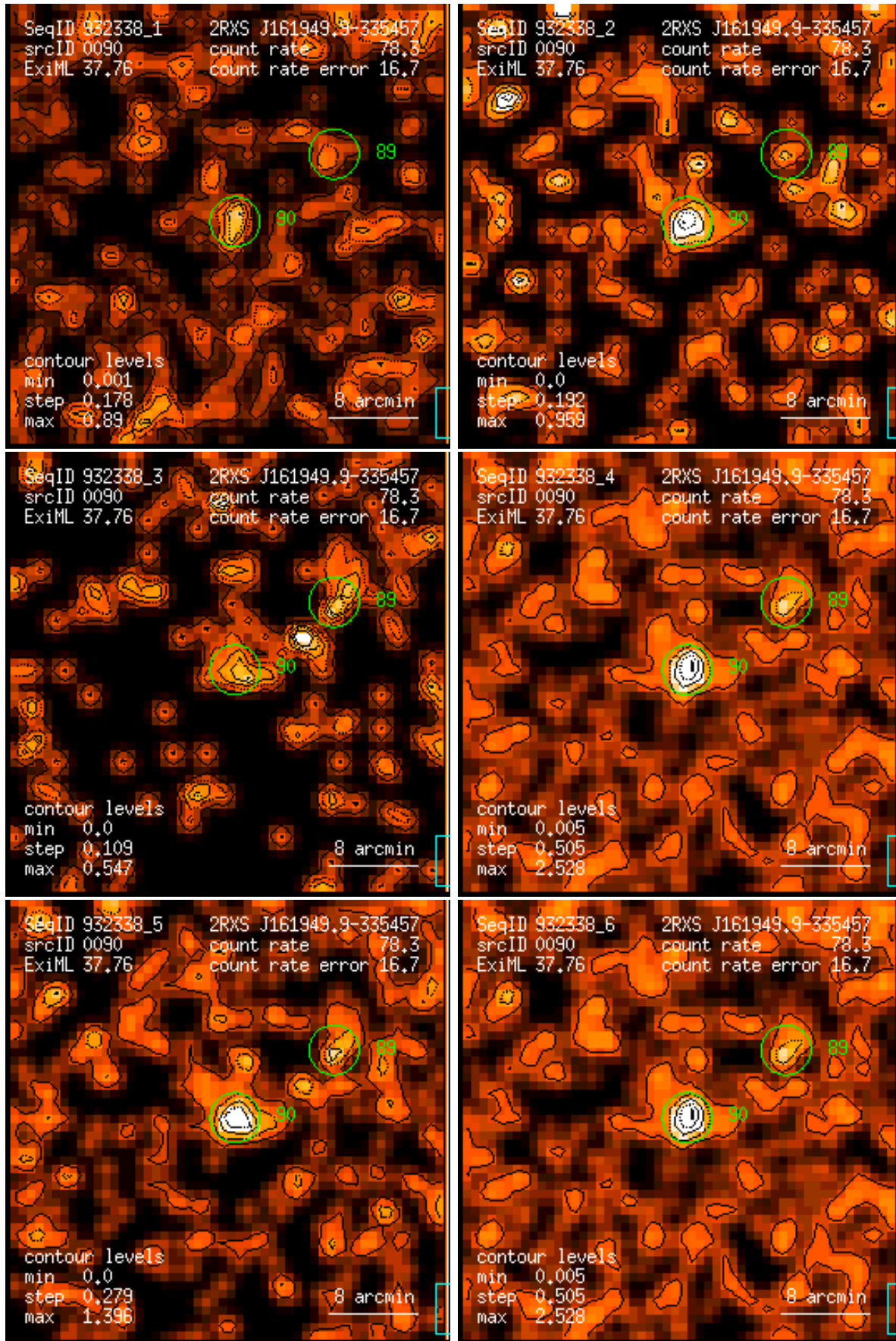
Figure 90: RASS 932338: detection 0090: band rate images, Gaussian filter: (1) PSPC channels 11 – 41, (2) 52 – 90, (3) 91 – 201, (4) 11 – 235, (5) 52 – 201, (6) 11 – 201. Broad band rates in counts/ks. Band rate contour levels in counts/ks/arcmin 2 .
