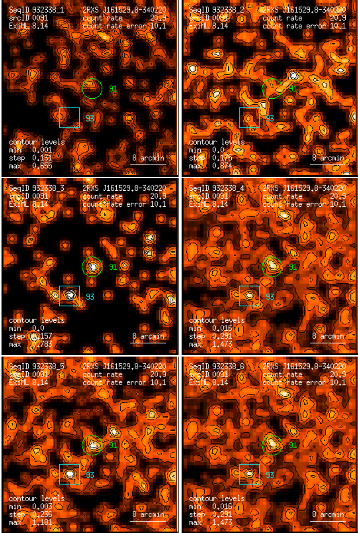
Figure 91: RASS 932338: detection 0091: band rate images, Gaussian filter: (1) PSPC channels 11 – 41, (2) 52 – 90, (3) 91 – 201, (4) 11 – 235, (5) 52 – 201, (6) 11 – 201. Broad band rates in counts/ks. Band rate contour levels in counts/ks/arcmin 2 .
