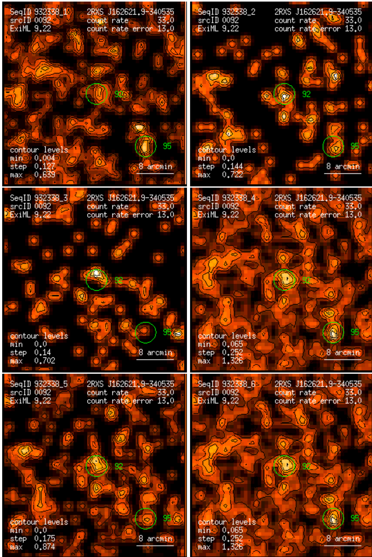
Figure 92: RASS 932338: detection 0092: band rate images, Gaussian filter: (1) PSPC channels 11 – 41, (2) 52 – 90, (3) 91 – 201, (4) 11 – 235, (5) 52 – 201, (6) 11 – 201. Broad band rates in counts/ks. Band rate contour levels in counts/ks/arcmin 2 .
