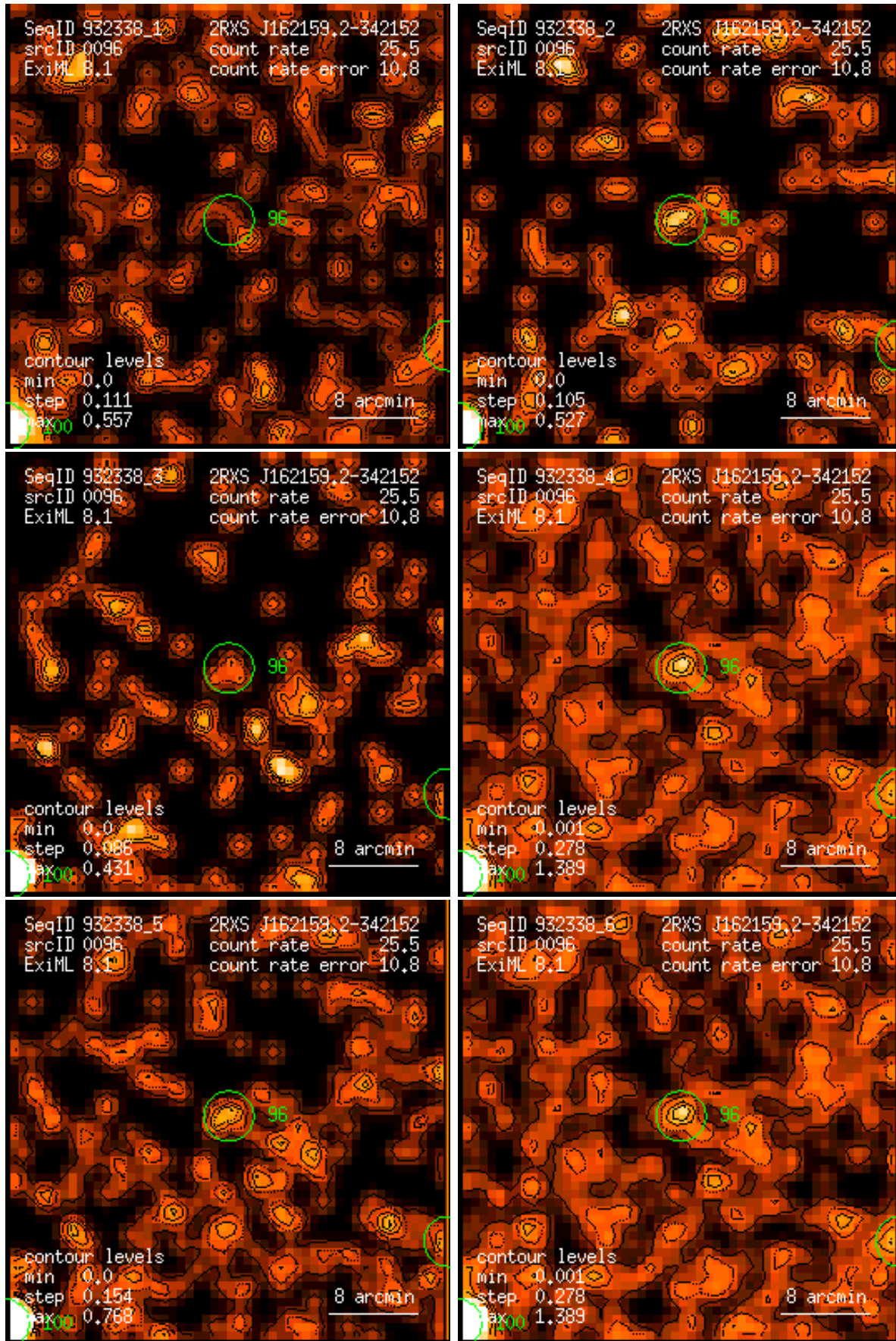
Figure 96: RASS 932338: detection 0096: band rate images, Gaussian filter: (1) PSPC channels 11 – 41, (2) 52 – 90, (3) 91 – 201, (4) 11 – 235, (5) 52 – 201, (6) 11 – 201. Broad band rates in counts/ks. Band rate contour levels in counts/ks/arcmin 2 .
