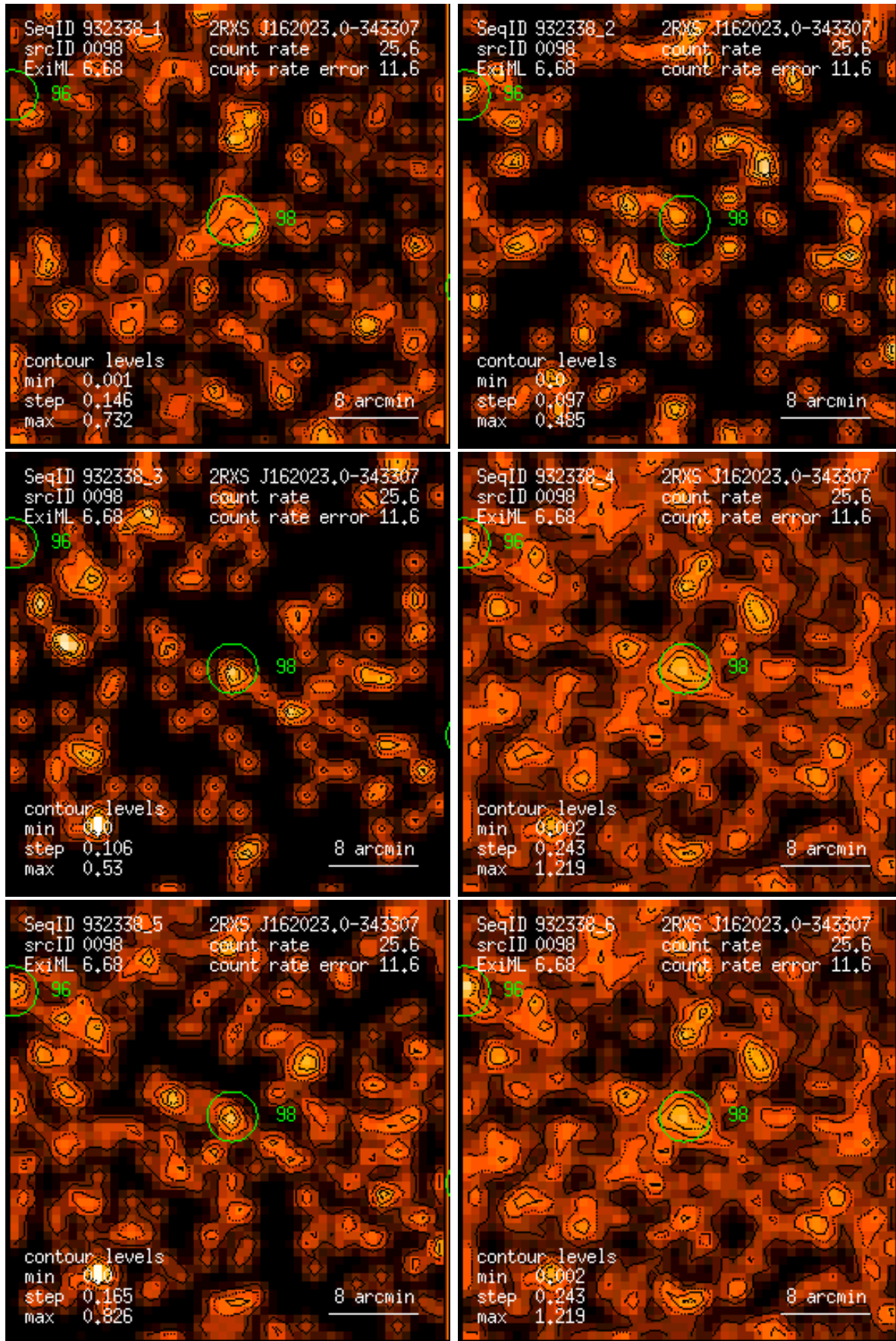
Figure 98: RASS 932338: detection 0098: band rate images, Gaussian filter: (1) PSPC channels 11 – 41, (2) 52 – 90, (3) 91 – 201, (4) 11 – 235, (5) 52 – 201, (6) 11 – 201. Broad band rates in counts/ks. Band rate contour levels in counts/ks/arcmin 2 .
