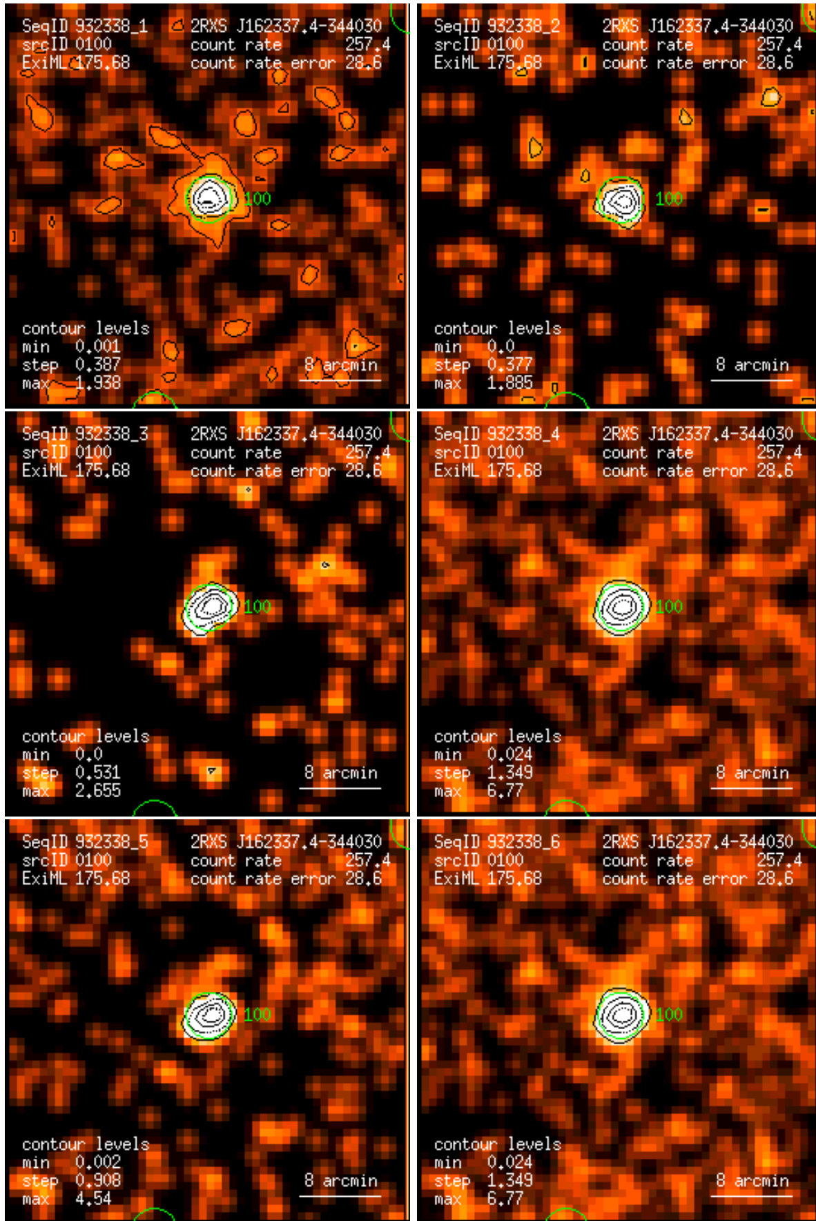
Figure 100: RASS 932338: detection 0100: band rate images, Gaussian filter: (1) PSPC channels 11 – 41, (2) 52 – 90, (3) 91 – 201, (4) 11 – 235, (5) 52 – 201, (6) 11 – 201. Broad band rates in counts/ks. Band rate contour levels in counts/ks/arcmin 2 .
