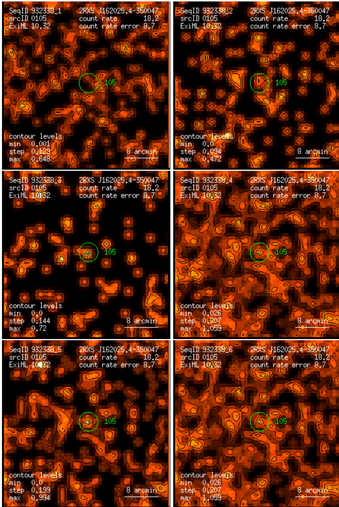
Figure 105: RASS 932338: detection 0105: band rate images, Gaussian filter: (1) PSPC channels 11 – 41, (2) 52 – 90, (3) 91 – 201, (4) 11 – 235, (5) 52 – 201, (6) 11 – 201. Broad band rates in counts/ks. Band rate contour levels in counts/ks/arcmin 2 .
