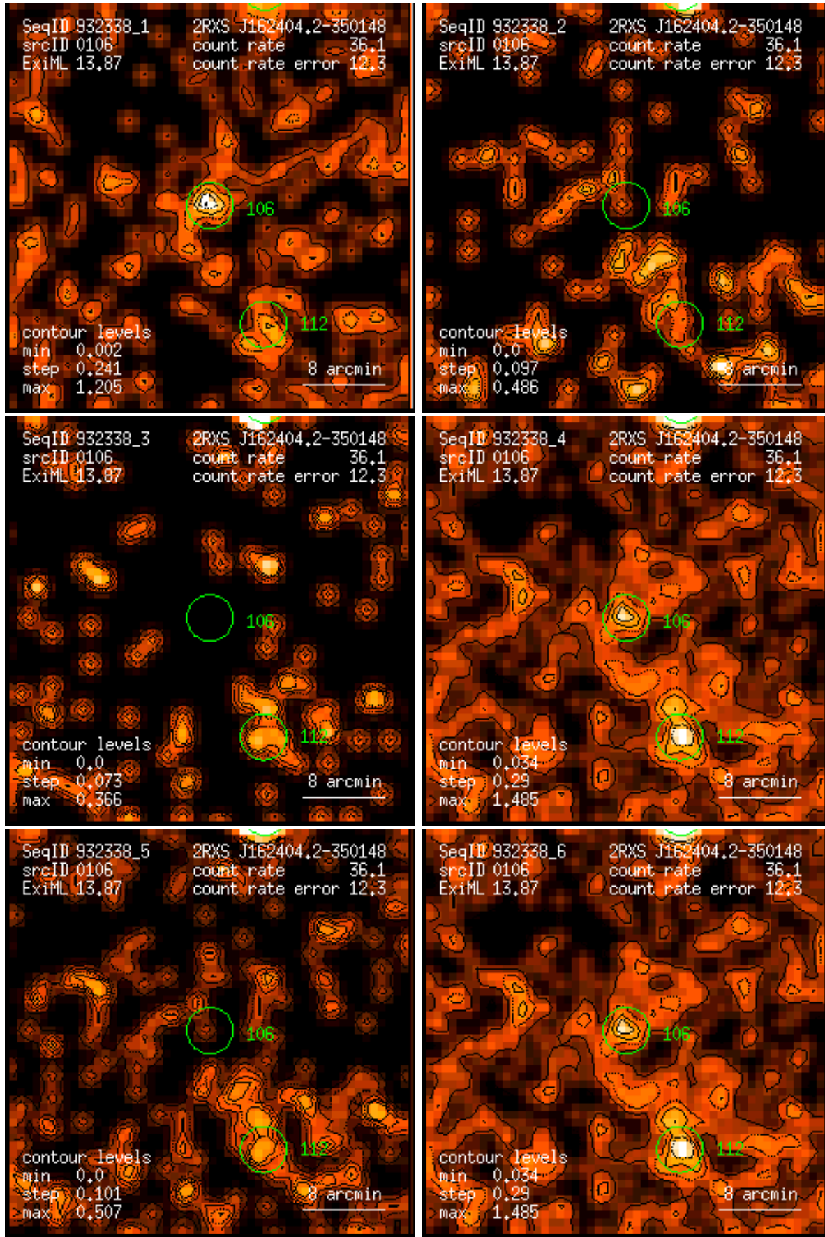
Figure 106: RASS 932338: detection 0106: band rate images, Gaussian filter: (1) PSPC channels 11 – 41, (2) 52 – 90, (3) 91 – 201, (4) 11 – 235, (5) 52 – 201, (6) 11 – 201. Broad band rates in counts/ks. Band rate contour levels in counts/ks/arcmin 2 .
