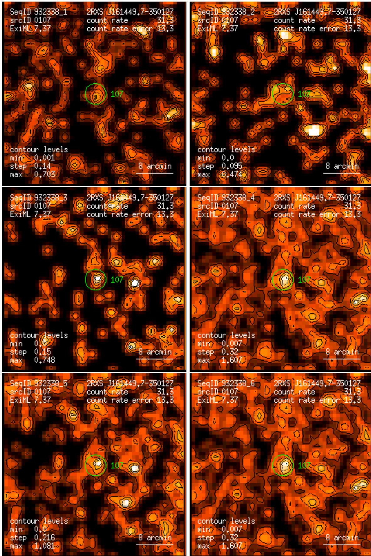
Figure 107: RASS 932338: detection 0107: band rate images, Gaussian filter: (1) PSPC channels 11 – 41, (2) 52 – 90, (3) 91 – 201, (4) 11 – 235, (5) 52 – 201, (6) 11 – 201. Broad band rates in counts/ks. Band rate contour levels in counts/ks/arcmin 2 .
