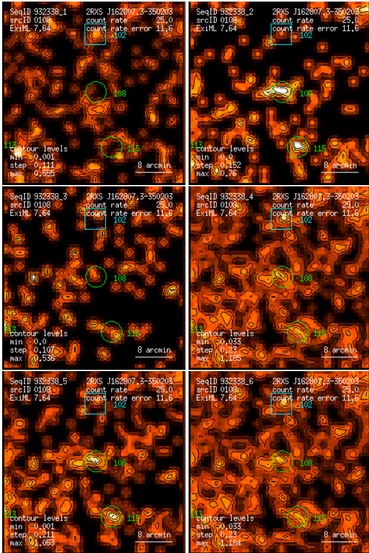
Figure 108: RASS 932338: detection 0108: band rate images, Gaussian filter: (1) PSPC channels 11 – 41, (2) 52 – 90, (3) 91 – 201, (4) 11 – 235, (5) 52 – 201, (6) 11 – 201. Broad band rates in counts/ks. Band rate contour levels in counts/ks/arcmin 2 .
