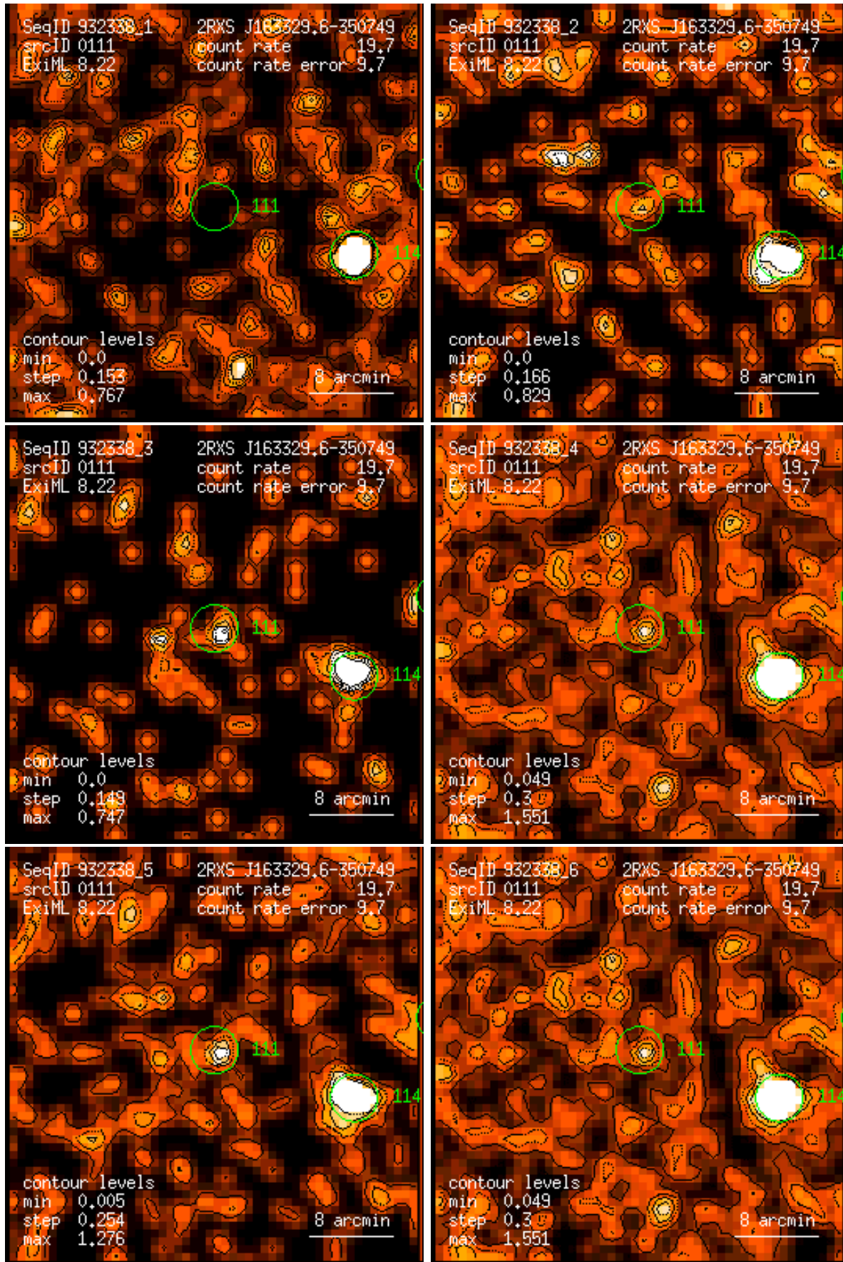
Figure 111: RASS 932338: detection 0111: band rate images, Gaussian filter: (1) PSPC channels 11 – 41, (2) 52 – 90, (3) 91 – 201, (4) 11 – 235, (5) 52 – 201, (6) 11 – 201. Broad band rates in counts/ks. Band rate contour levels in counts/ks/arcmin 2 .
