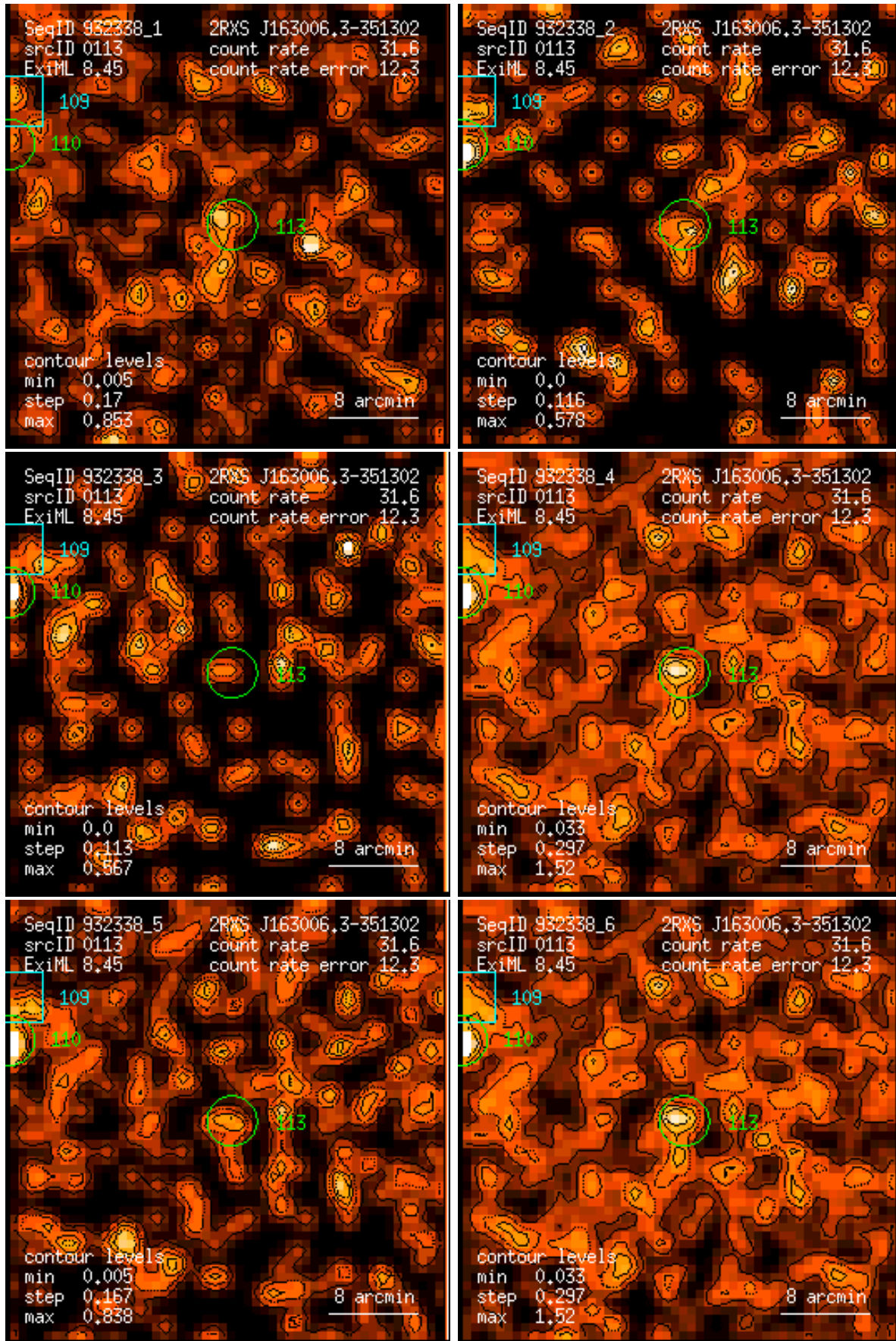
Figure 113: RASS 932338: detection 0113: band rate images, Gaussian filter: (1) PSPC channels 11 – 41, (2) 52 – 90, (3) 91 – 201, (4) 11 – 235, (5) 52 – 201, (6) 11 – 201. Broad band rates in counts/ks. Band rate contour levels in counts/ks/arcmin 2 .
