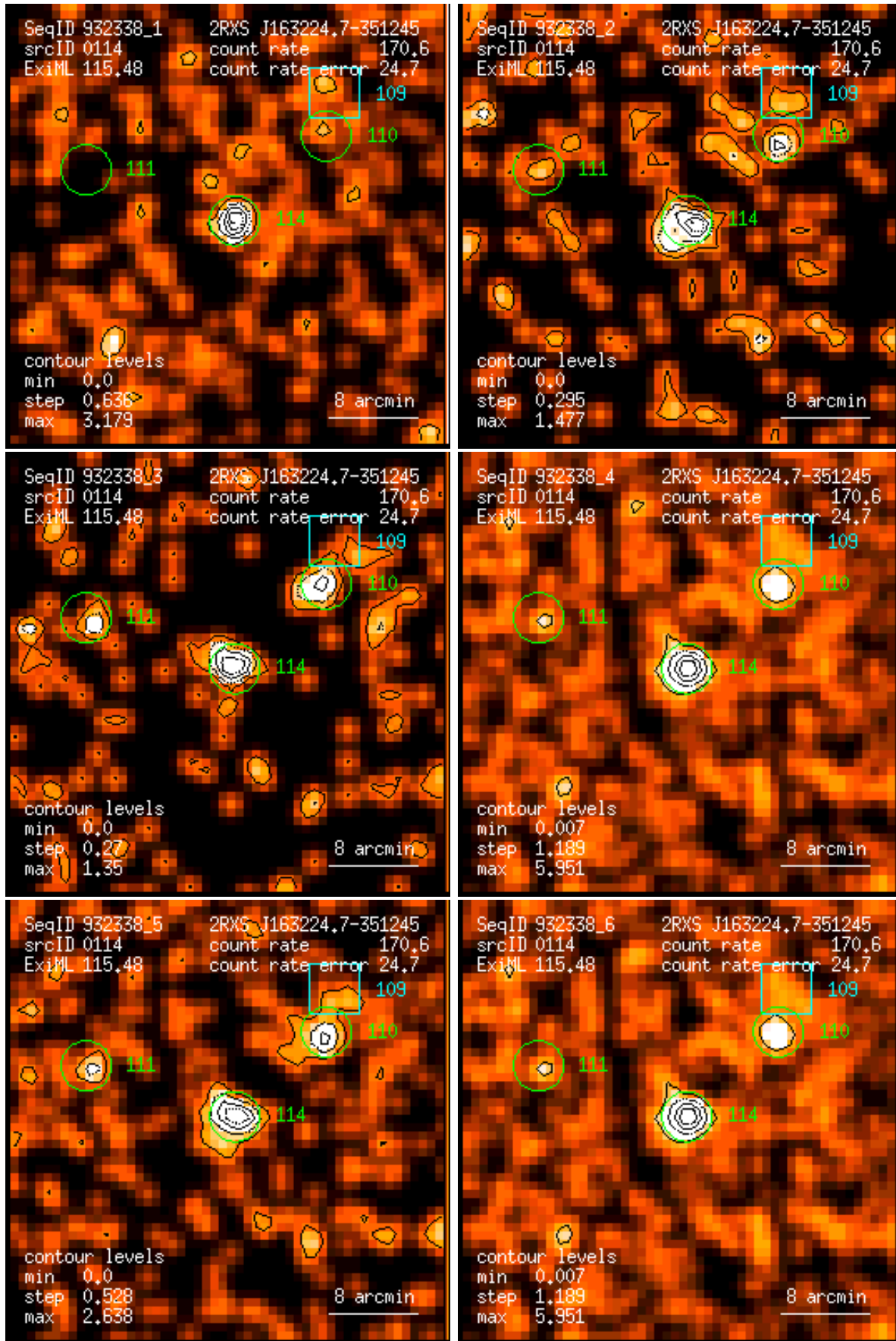
Figure 114: RASS 932338: detection 0114: band rate images, Gaussian filter: (1) PSPC channels 11 – 41, (2) 52 – 90, (3) 91 – 201, (4) 11 – 235, (5) 52 – 201, (6) 11 – 201. Broad band rates in counts/ks. Band rate contour levels in counts/ks/arcmin 2 .
