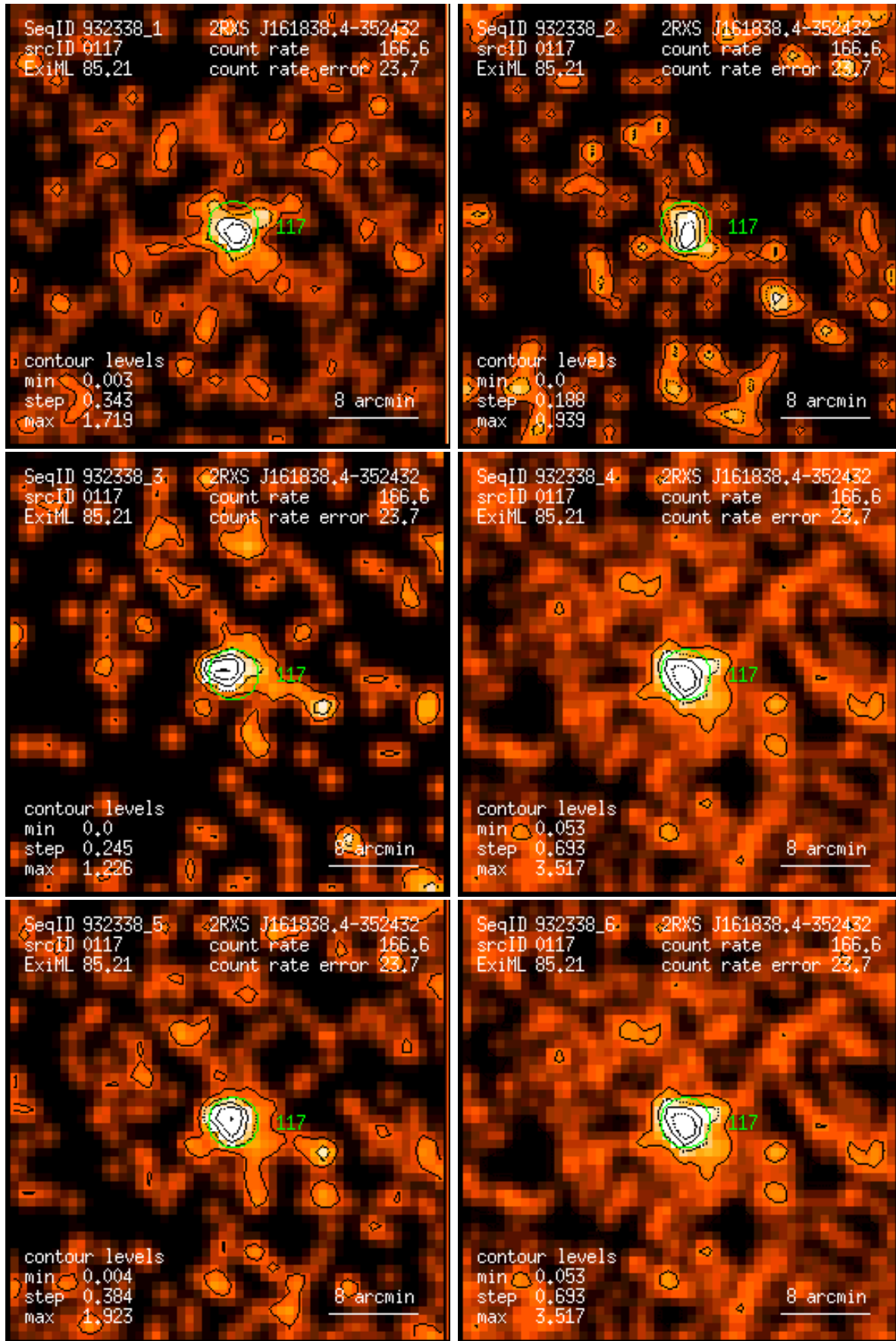
Figure 117: RASS 932338: detection 0117: band rate images, Gaussian filter: (1) PSPC channels 11 – 41, (2) 52 – 90, (3) 91 – 201, (4) 11 – 235, (5) 52 – 201, (6) 11 – 201. Broad band rates in counts/ks. Band rate contour levels in counts/ks/arcmin 2 .
