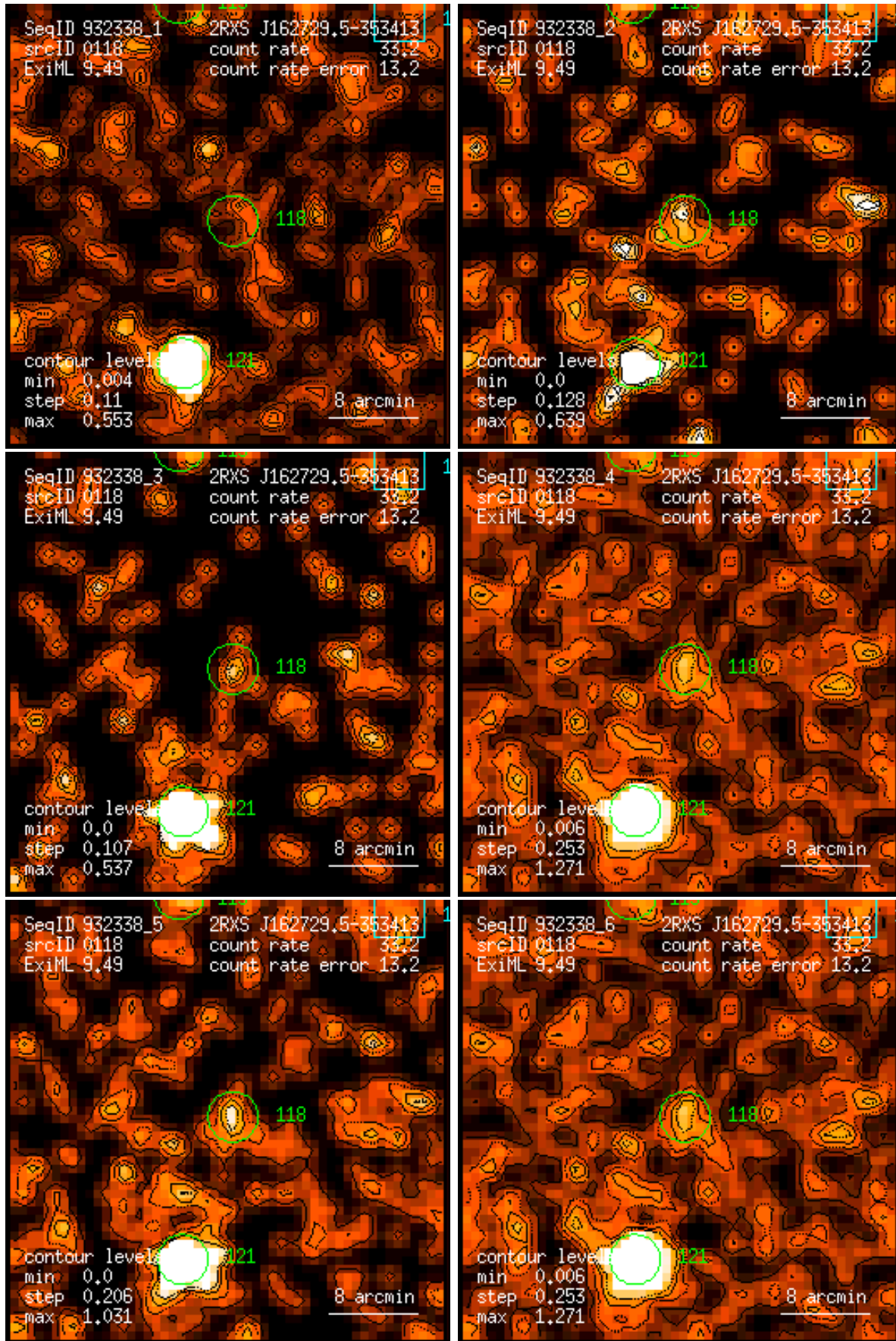
Figure 118: RASS 932338: detection 0118: band rate images, Gaussian filter: (1) PSPC channels 11 – 41, (2) 52 – 90, (3) 91 – 201, (4) 11 – 235, (5) 52 – 201, (6) 11 – 201. Broad band rates in counts/ks. Band rate contour levels in counts/ks/arcmin 2 .
