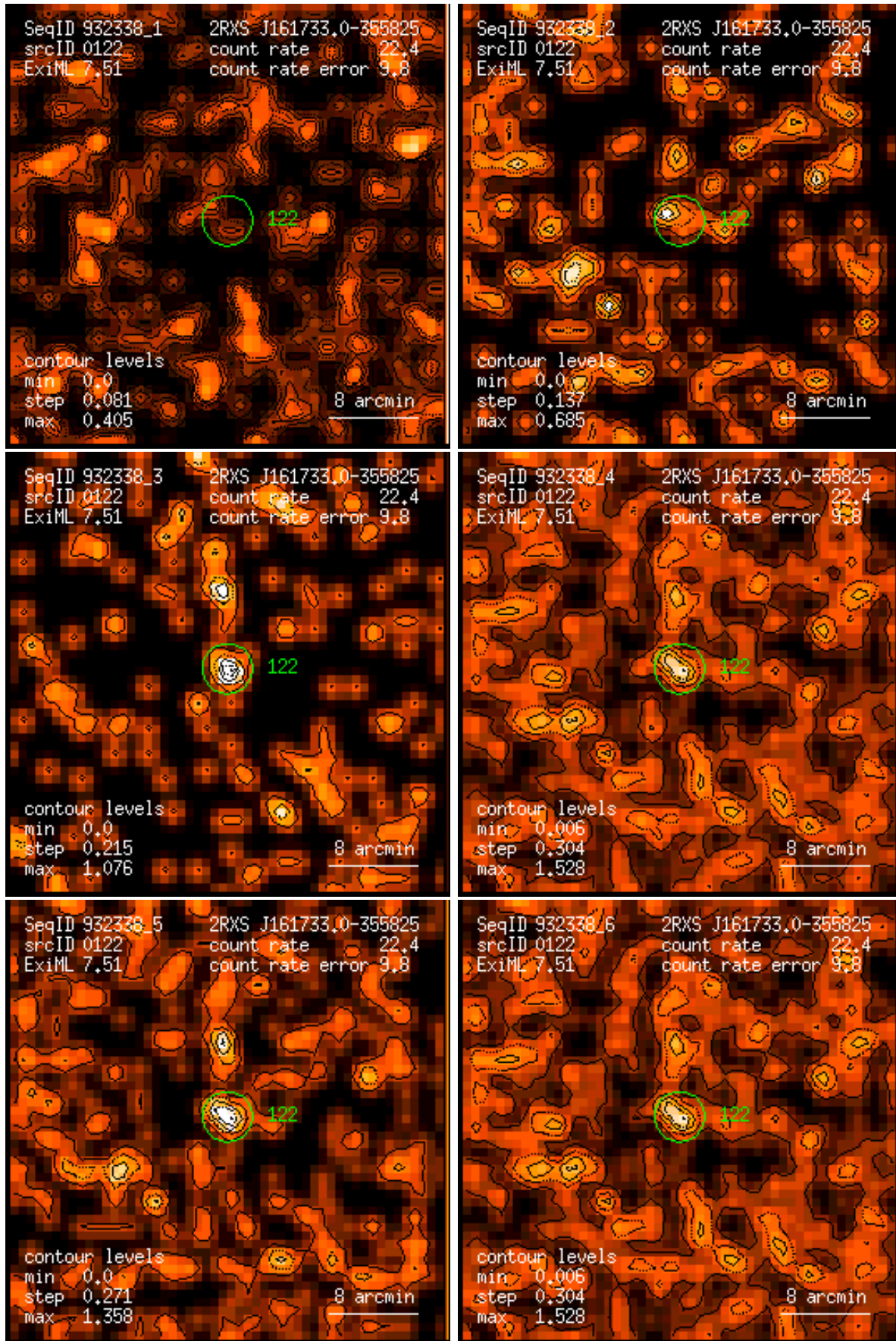
Figure 122: RASS 932338: detection 0122: band rate images, Gaussian filter: (1) PSPC channels 11 – 41, (2) 52 – 90, (3) 91 – 201, (4) 11 – 235, (5) 52 – 201, (6) 11 – 201. Broad band rates in counts/ks. Band rate contour levels in counts/ks/arcmin 2 .
