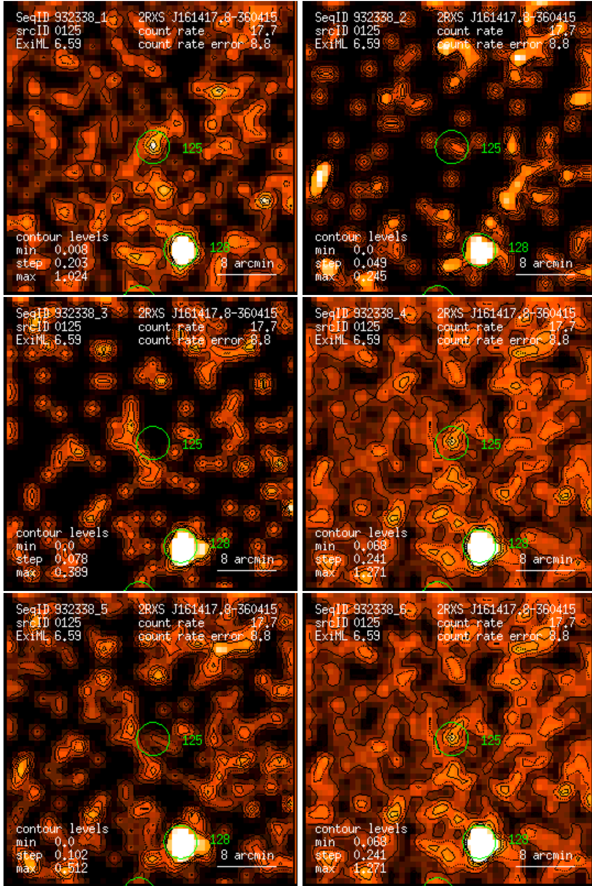
Figure 125: RASS 932338: detection 0125: band rate images, Gaussian filter: (1) PSPC channels 11 – 41, (2) 52 – 90, (3) 91 – 201, (4) 11 – 235, (5) 52 – 201, (6) 11 – 201. Broad band rates in counts/ks. Band rate contour levels in counts/ks/arcmin 2 .
