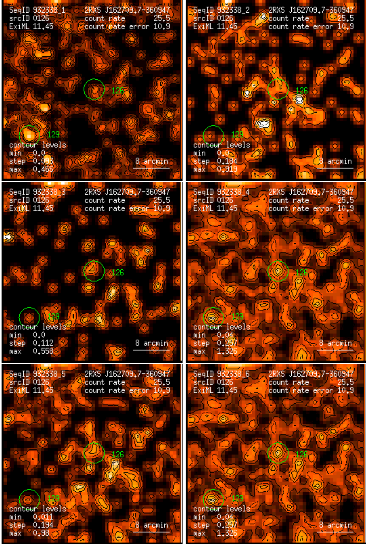
Figure 126: RASS 932338: detection 0126: band rate images, Gaussian filter: (1) PSPC channels 11 – 41, (2) 52 – 90, (3) 91 – 201, (4) 11 – 235, (5) 52 – 201, (6) 11 – 201. Broad band rates in counts/ks. Band rate contour levels in counts/ks/arcmin 2 .
