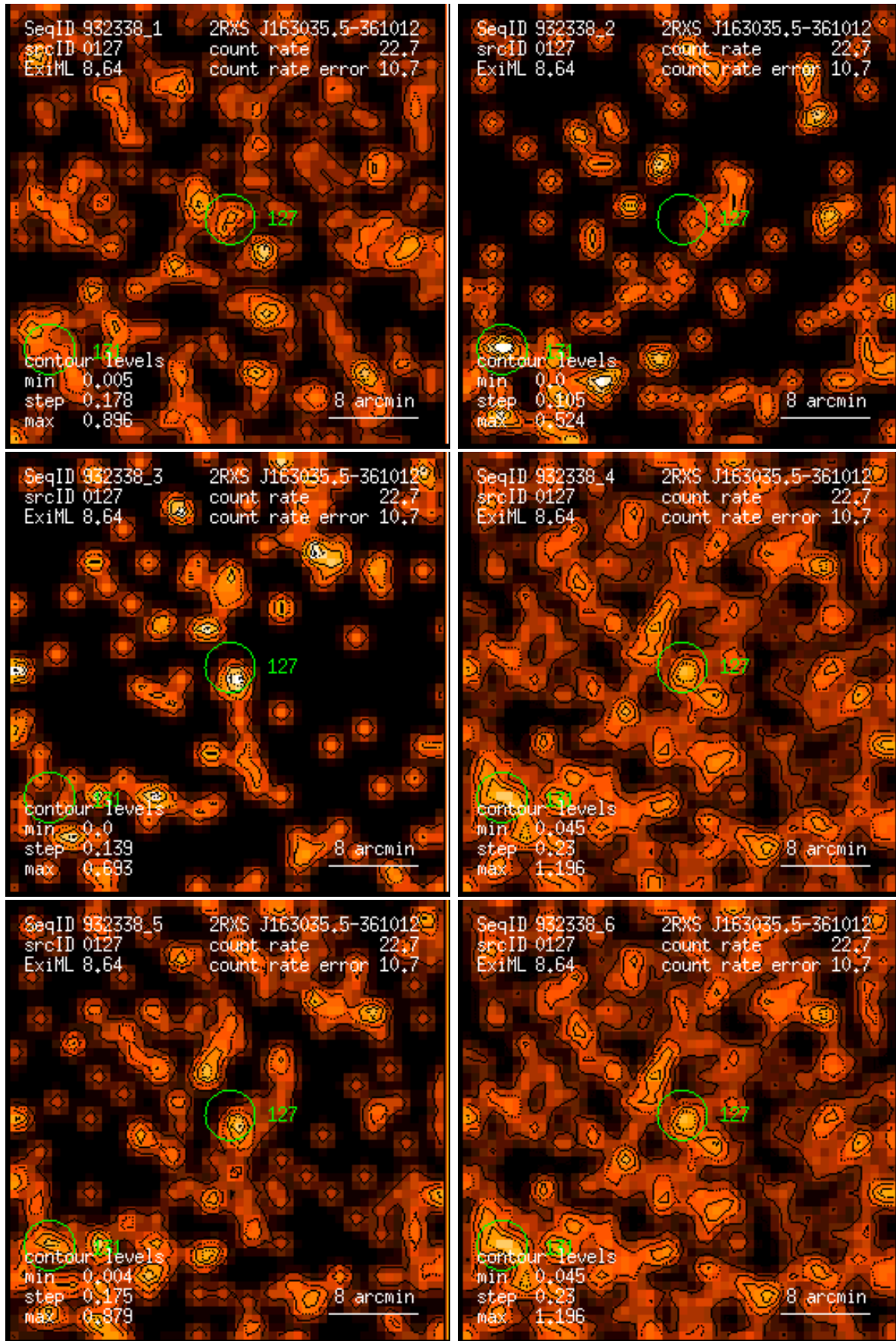
Figure 127: RASS 932338: detection 0127: band rate images, Gaussian filter: (1) PSPC channels 11 – 41, (2) 52 – 90, (3) 91 – 201, (4) 11 – 235, (5) 52 – 201, (6) 11 – 201. Broad band rates in counts/ks. Band rate contour levels in counts/ks/arcmin 2 .
