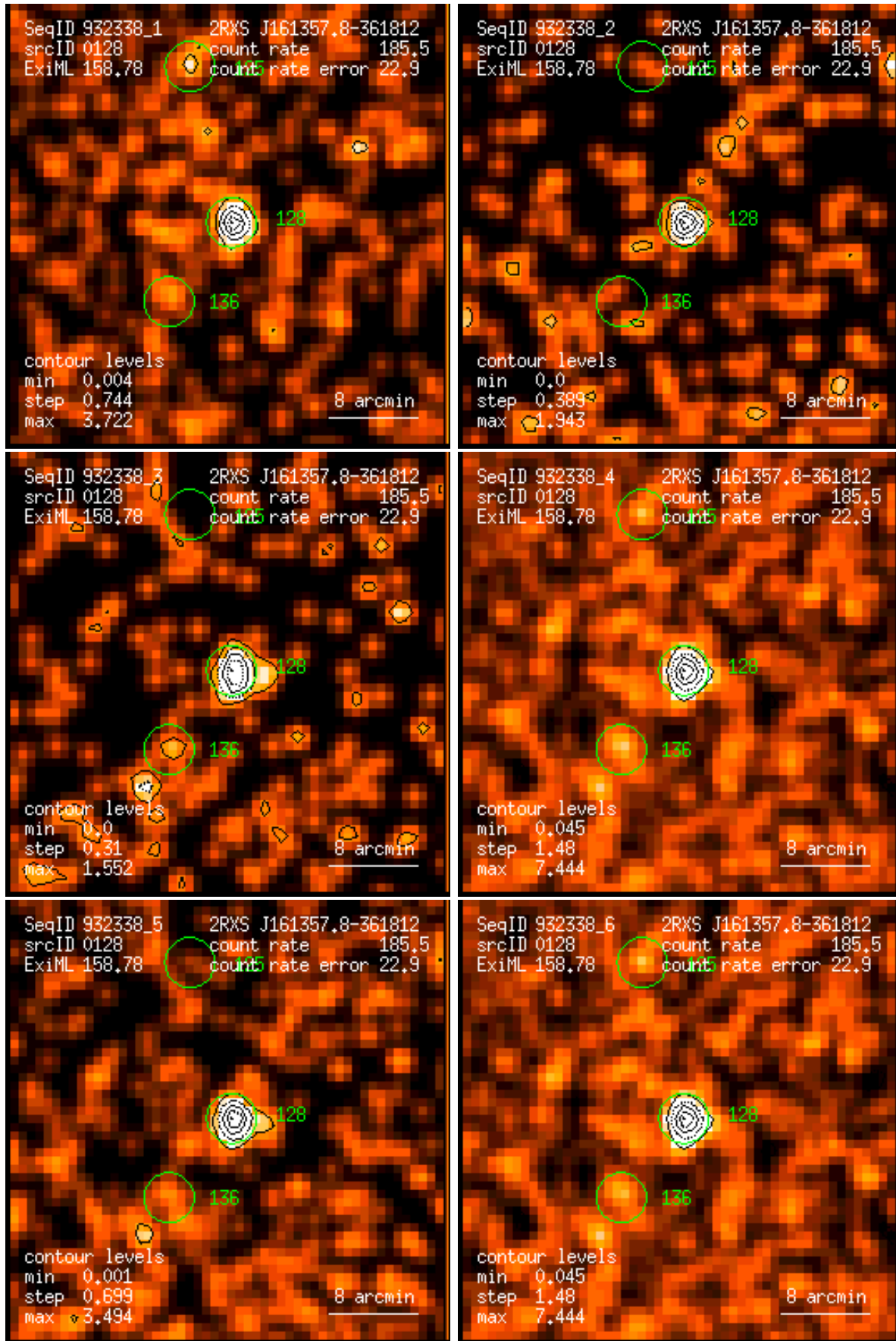
Figure 128: RASS 932338: detection 0128: band rate images, Gaussian filter: (1) PSPC channels 11 – 41, (2) 52 – 90, (3) 91 – 201, (4) 11 – 235, (5) 52 – 201, (6) 11 – 201. Broad band rates in counts/ks. Band rate contour levels in counts/ks/arcmin 2 .
