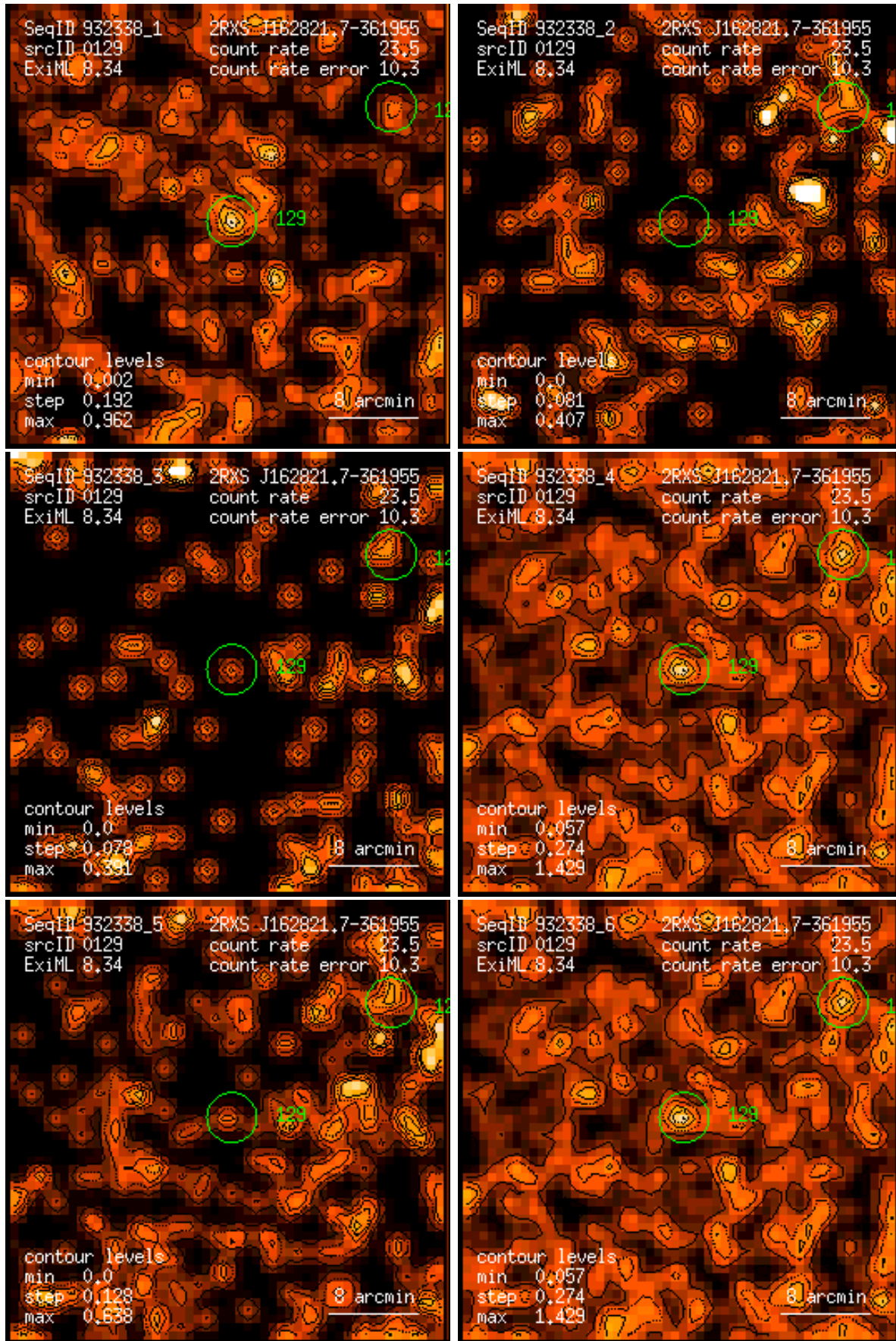
Figure 129: RASS 932338: detection 0129: band rate images, Gaussian filter: (1) PSPC channels 11 – 41, (2) 52 – 90, (3) 91 – 201, (4) 11 – 235, (5) 52 – 201, (6) 11 – 201. Broad band rates in counts/ks. Band rate contour levels in counts/ks/arcmin 2 .
