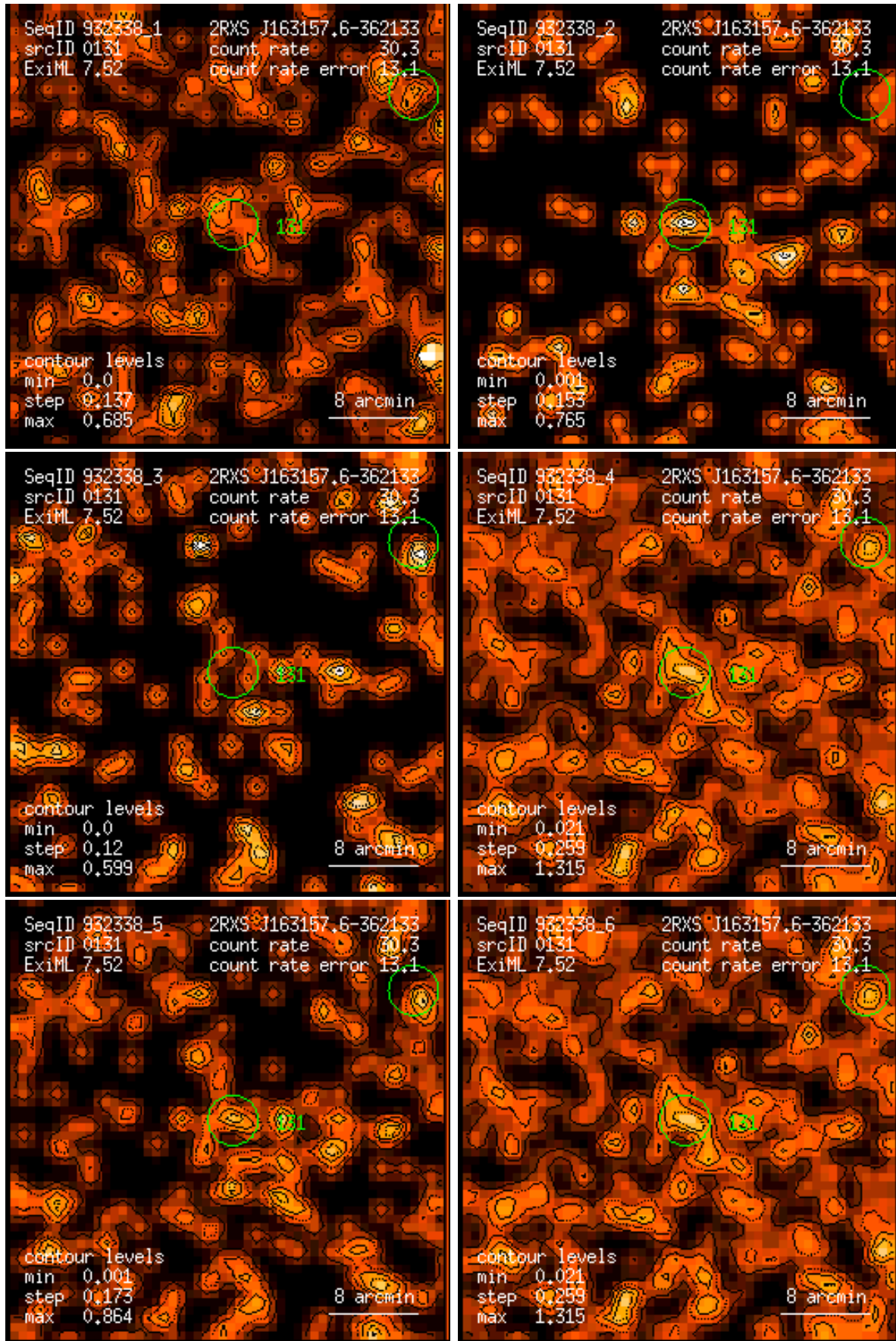
Figure 131: RASS 932338: detection 0131: band rate images, Gaussian filter: (1) PSPC channels 11 – 41, (2) 52 – 90, (3) 91 – 201, (4) 11 – 235, (5) 52 – 201, (6) 11 – 201. Broad band rates in counts/ks. Band rate contour levels in counts/ks/arcmin 2 .
