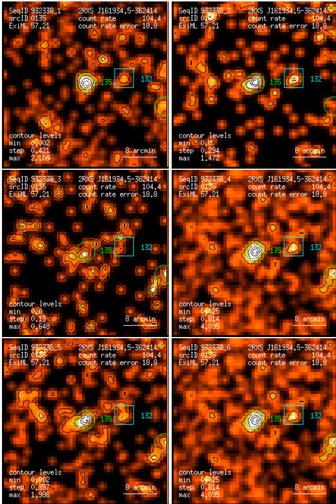
Figure 135: RASS 932338: detection 0135: band rate images, Gaussian filter: (1) PSPC channels 11 – 41, (2) 52 – 90, (3) 91 – 201, (4) 11 – 235, (5) 52 – 201, (6) 11 – 201. Broad band rates in counts/ks. Band rate contour levels in counts/ks/arcmin 2 .
