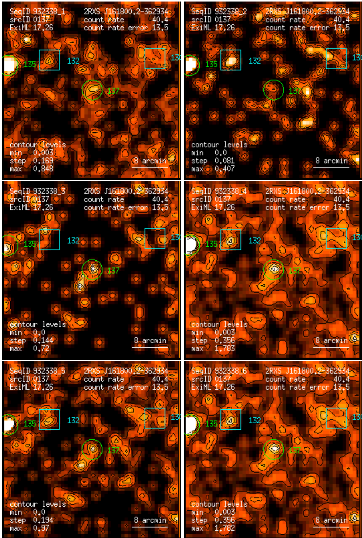
Figure 137: RASS 932338: detection 0137: band rate images, Gaussian filter: (1) PSPC channels 11 – 41, (2) 52 – 90, (3) 91 – 201, (4) 11 – 235, (5) 52 – 201, (6) 11 – 201. Broad band rates in counts/ks. Band rate contour levels in counts/ks/arcmin 2 .
