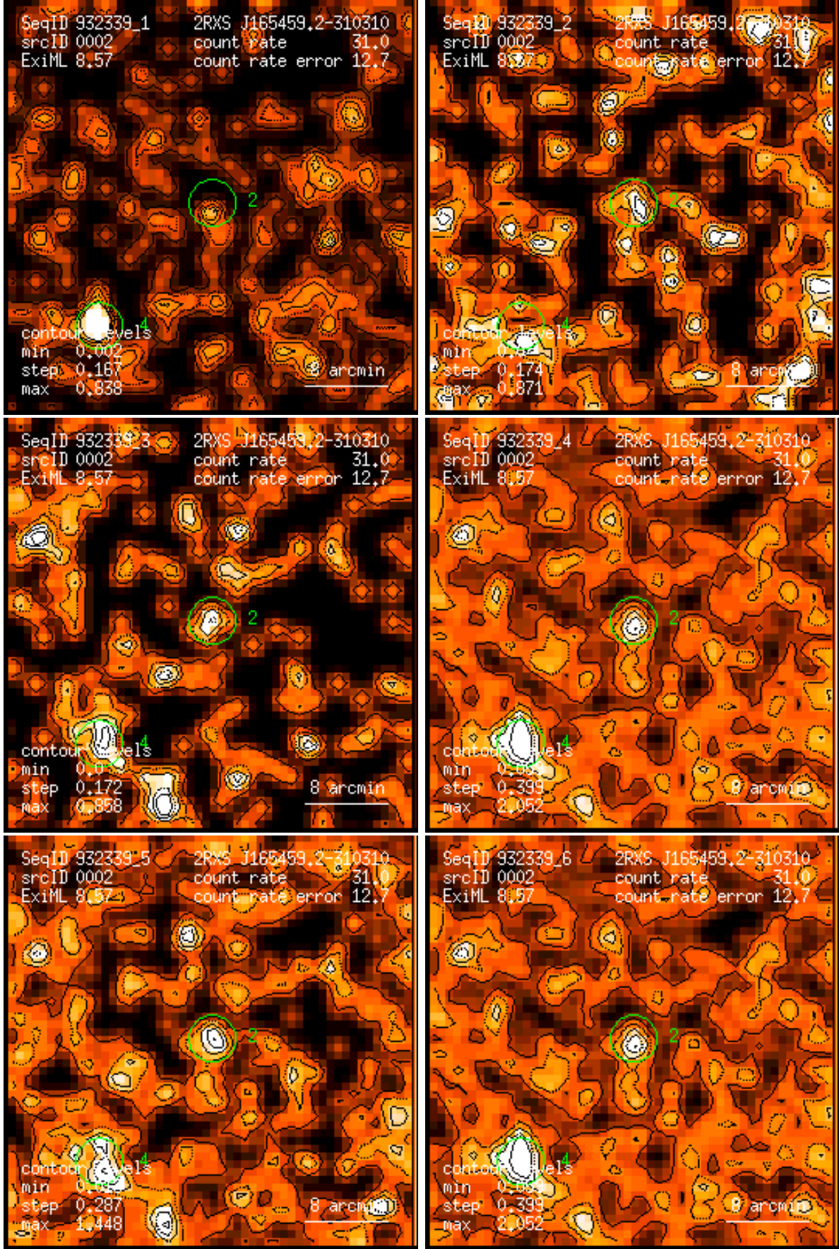
Figure 2: RASS 932339: detection 0002: band rate images, Gaussian filter: (1) PSPC channels 11 – 41, (2) 52 – 90, (3) 91 – 201, (4) 11 – 235, (5) 52 – 201, (6) 11 – 201. Broad band rates in counts/ks. Band rate contour levels in counts/ks/arcmin 2 .
