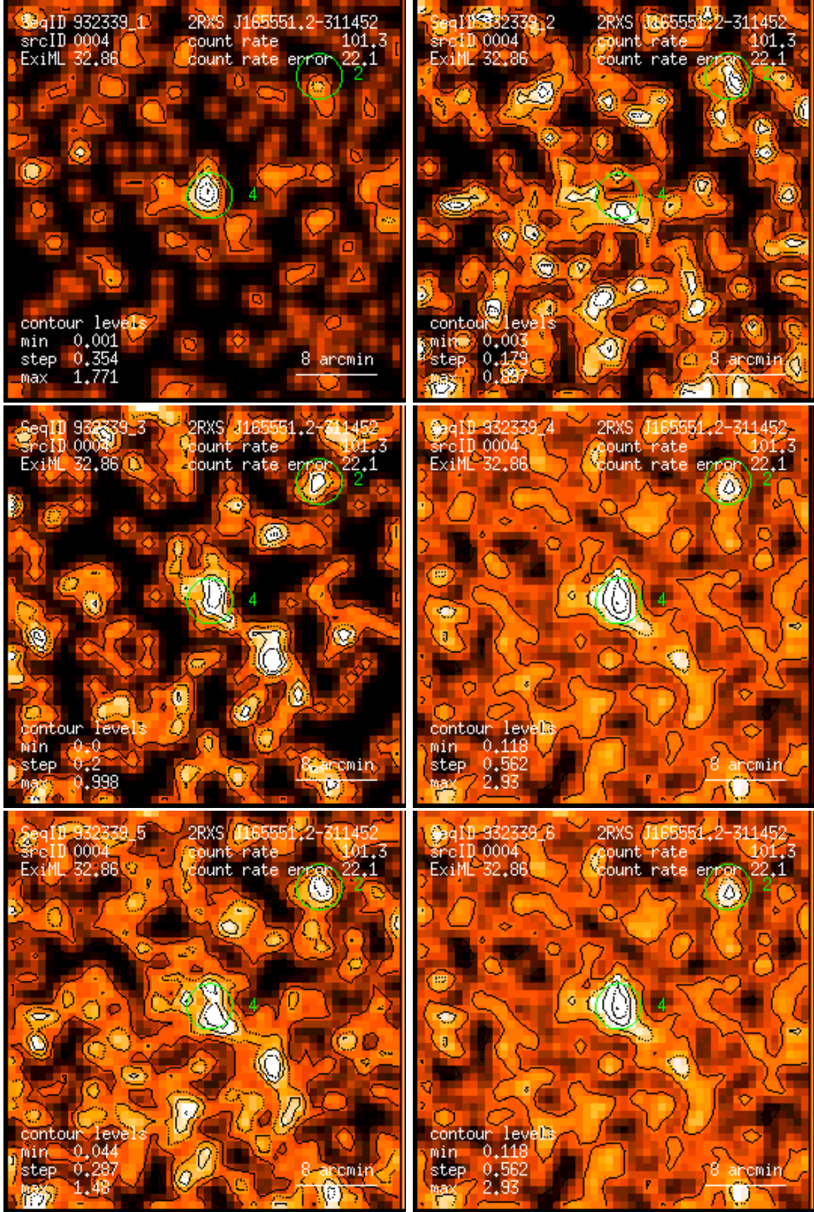
Figure 4: RASS 932339: detection 0004: band rate images, Gaussian filter: (1) PSPC channels 11 – 41, (2) 52 – 90, (3) 91 – 201, (4) 11 – 235, (5) 52 – 201, (6) 11 – 201. Broad band rates in counts/ks. Band rate contour levels in counts/ks/arcmin 2 .
