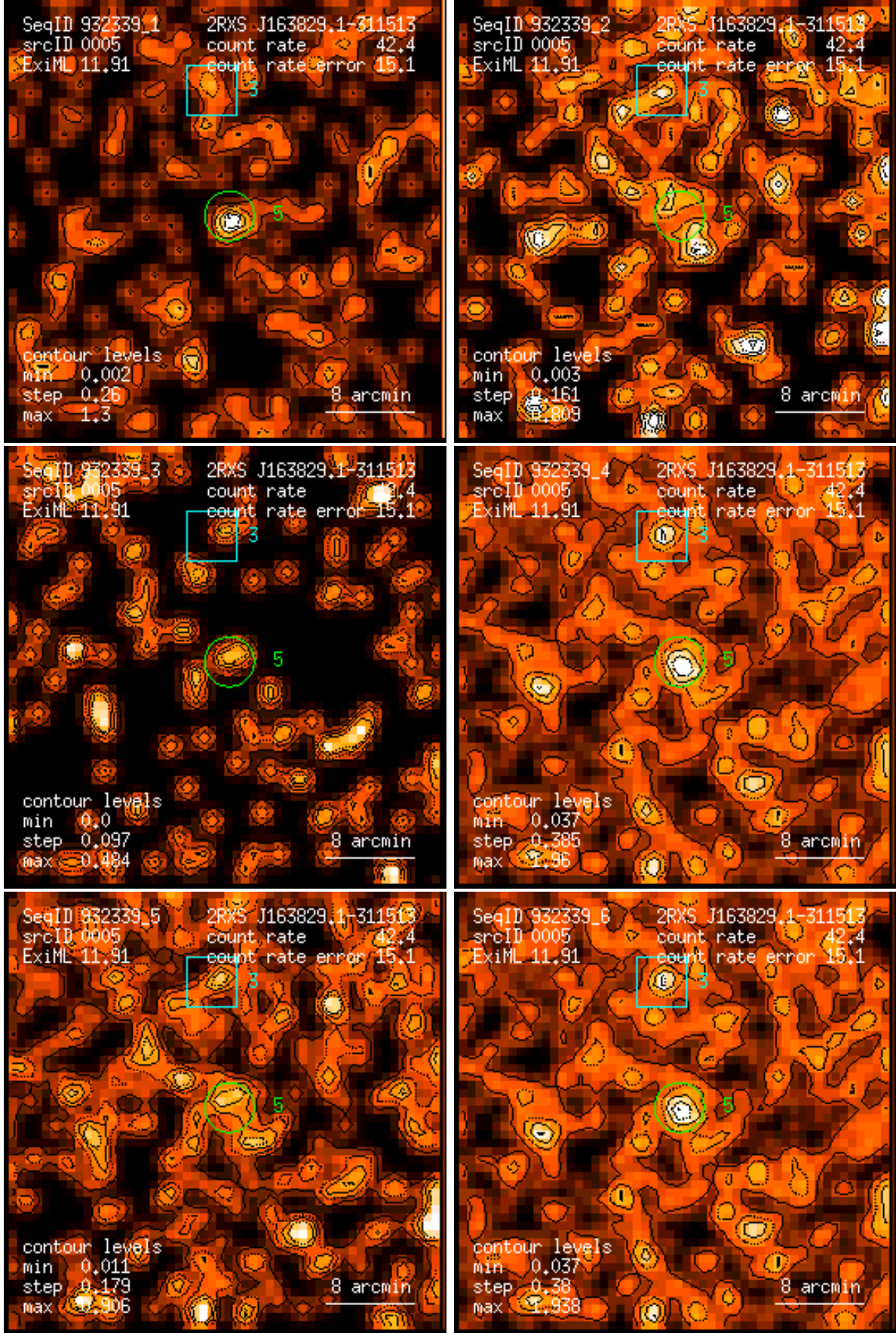
Figure 5: RASS 932339: detection 0005: band rate images, Gaussian filter: (1) PSPC channels 11 – 41, (2) 52 – 90, (3) 91 – 201, (4) 11 – 235, (5) 52 – 201, (6) 11 – 201. Broad band rates in counts/ks. Band rate contour levels in counts/ks/arcmin 2 .
