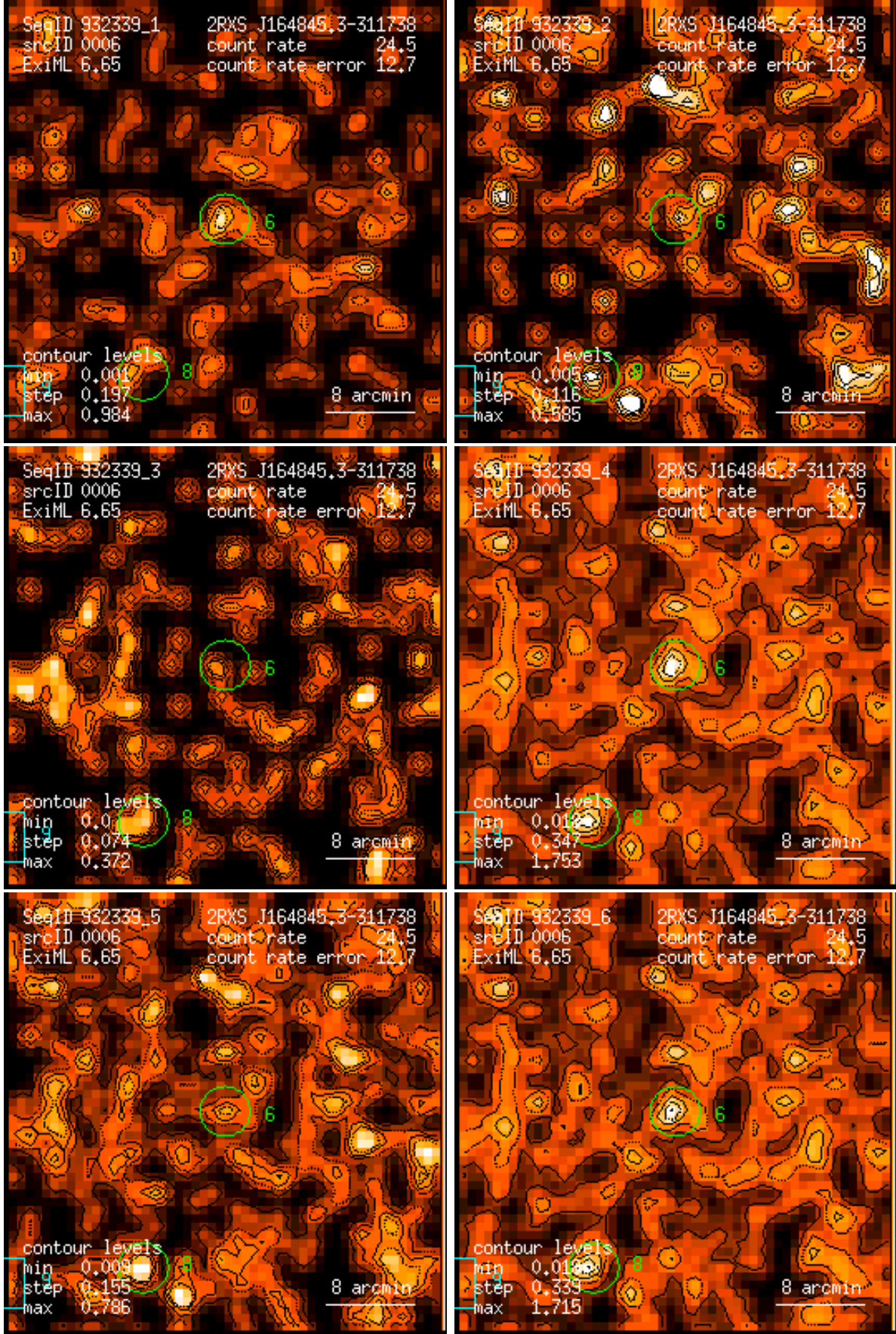
Figure 6: RASS 932339: detection 0006: band rate images, Gaussian filter: (1) PSPC channels 11 – 41, (2) 52 – 90, (3) 91 – 201, (4) 11 – 235, (5) 52 – 201, (6) 11 – 201. Broad band rates in counts/ks. Band rate contour levels in counts/ks/arcmin 2 .
