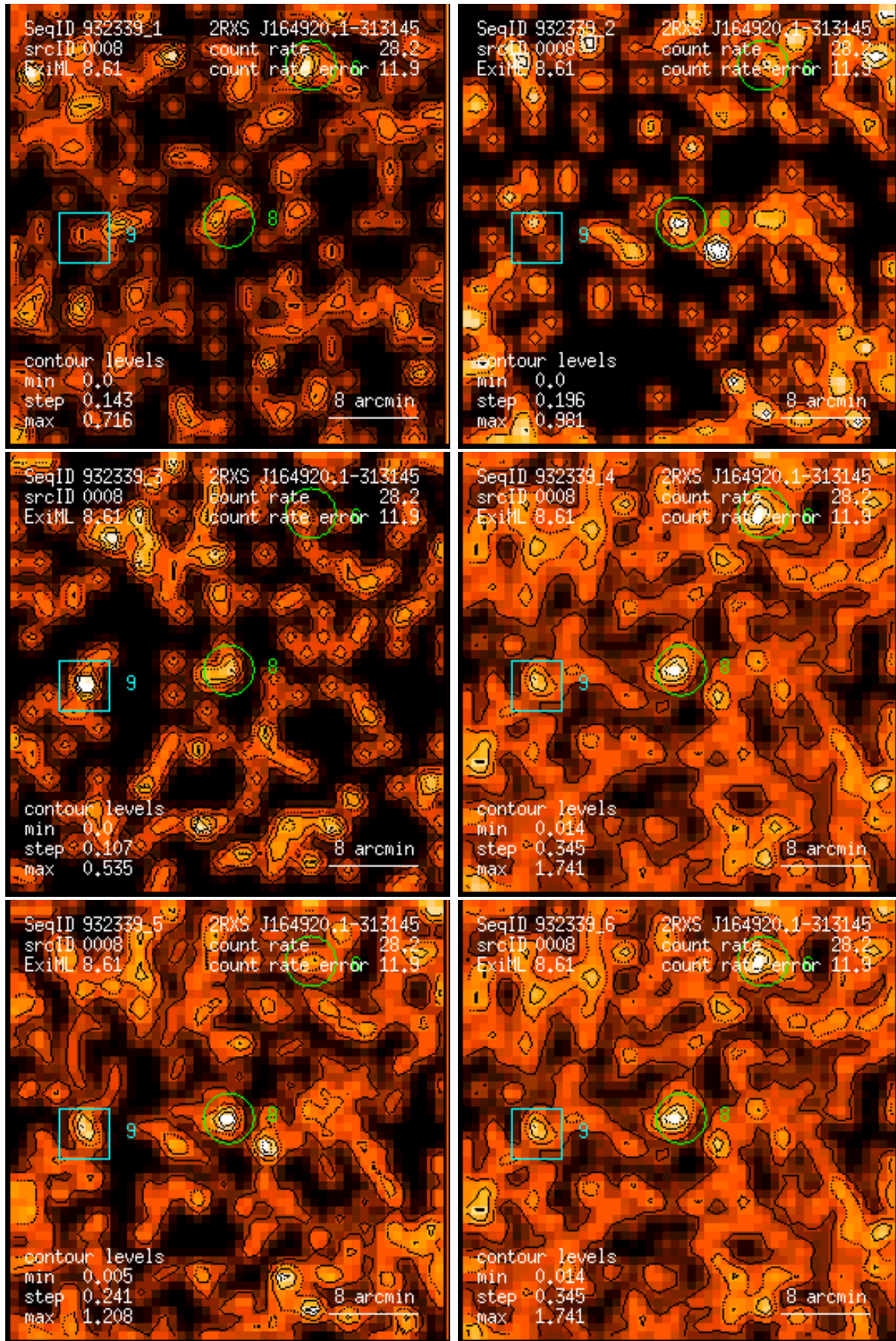
Figure 8: RASS 932339: detection 0008: band rate images, Gaussian filter: (1) PSPC channels 11 – 41, (2) 52 – 90, (3) 91 – 201, (4) 11 – 235, (5) 52 – 201, (6) 11 – 201. Broad band rates in counts/ks. Band rate contour levels in counts/ks/arcmin 2 .
