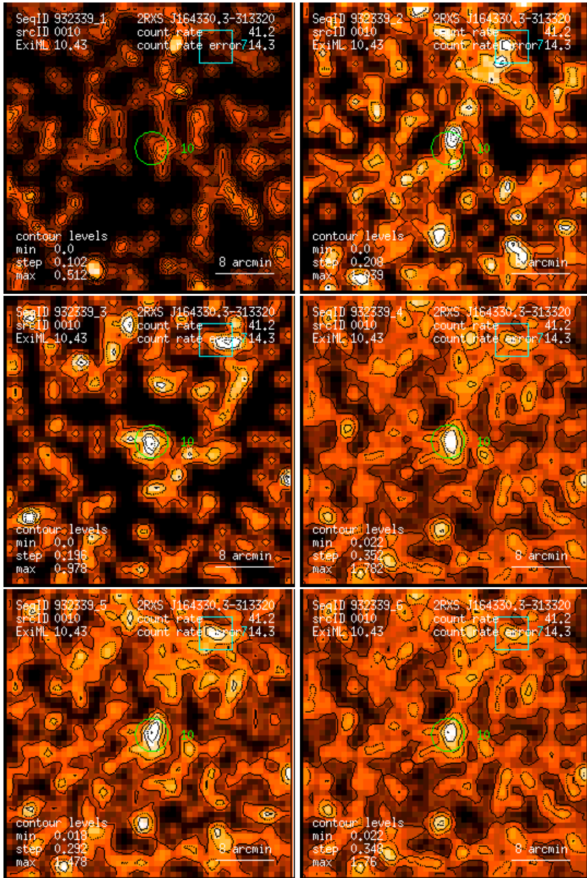
Figure 10: RASS 932339: detection 0010: band rate images, Gaussian filter: (1) PSPC channels 11 – 41, (2) 52 – 90, (3) 91 – 201, (4) 11 – 235, (5) 52 – 201, (6) 11 – 201. Broad band rates in counts/ks. Band rate contour levels in counts/ks/arcmin 2 .
