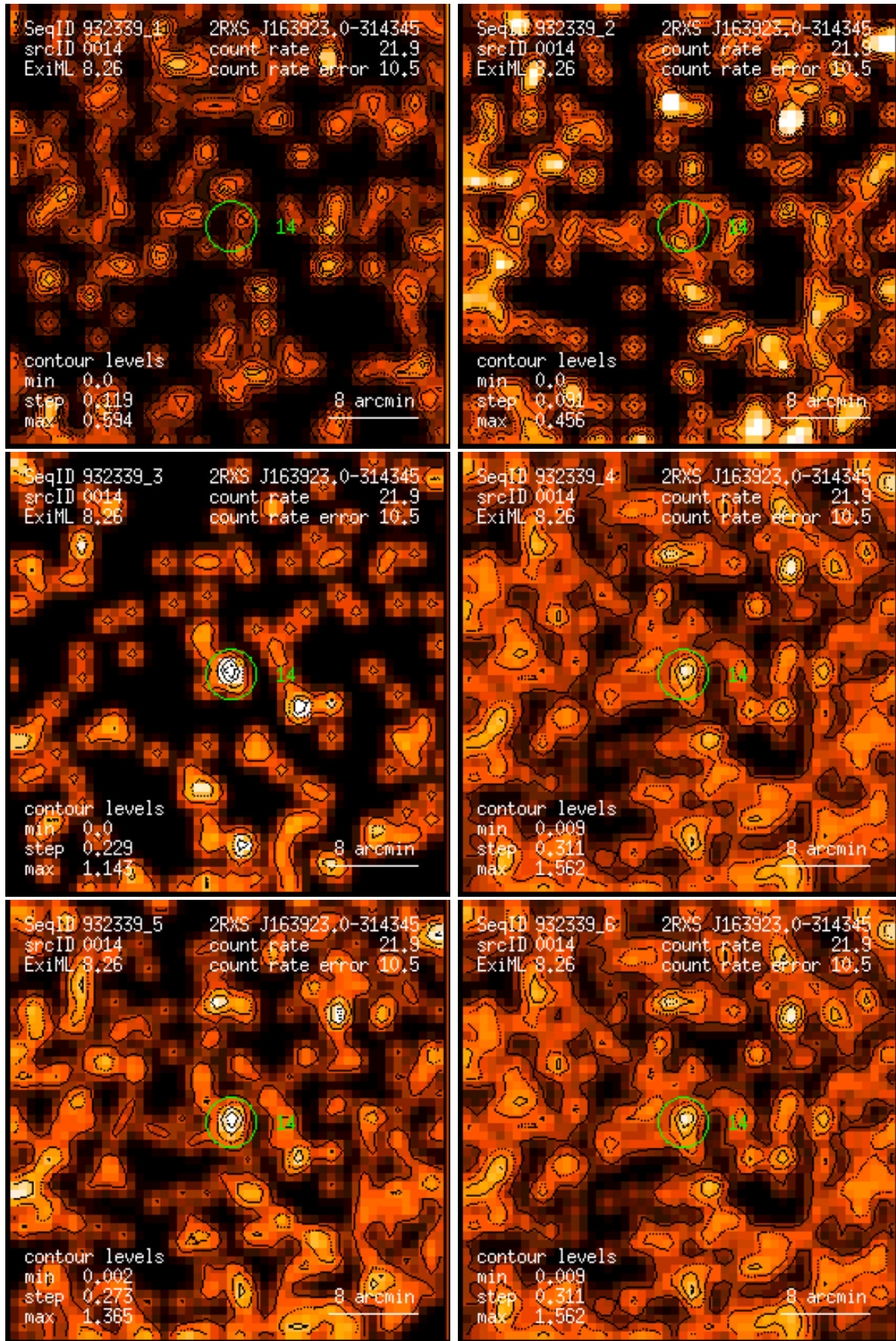
Figure 14: RASS 932339: detection 0014: band rate images, Gaussian filter: (1) PSPC channels 11 – 41, (2) 52 – 90, (3) 91 – 201, (4) 11 – 235, (5) 52 – 201, (6) 11 – 201. Broad band rates in counts/ks. Band rate contour levels in counts/ks/arcmin 2 .
