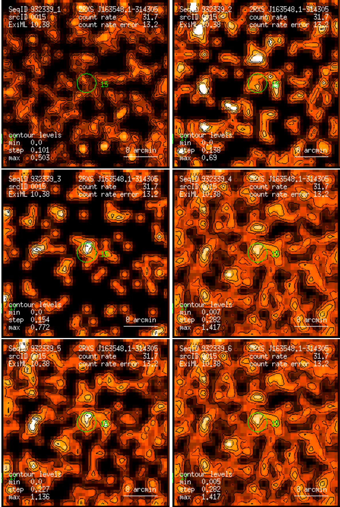
Figure 15: RASS 932339: detection 0015: band rate images, Gaussian filter: (1) PSPC channels 11 – 41, (2) 52 – 90, (3) 91 – 201, (4) 11 – 235, (5) 52 – 201, (6) 11 – 201. Broad band rates in counts/ks. Band rate contour levels in counts/ks/arcmin 2 .
